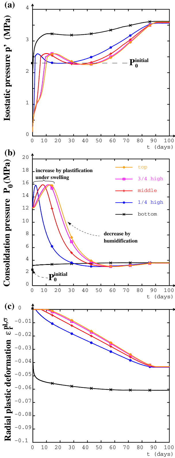
Figure 4: Temporal evolution at different vertical positions, for an initial consolidation pressure P_0 = 2.3 MPa. It shows how plastic deformation \varepsilon_r^{pl,\sigma} begins when radial stress \sigma_{rr} exceeds P_0 . Black squares indicate initial point.
