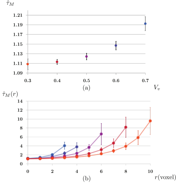
Fig. 9: (a) \hat{\tau}_M , the M-tortuosity value, as a function of V_v , the solid volume fraction of Boolean models of spheres of radius R = 10 , and (b) M-tortuosity-by-iterative-erosions , \hat{\tau}_M(r) , for each model defined by V_v . Confidence intervals, with confidence level at 95 %, are represented by vertical bars.
