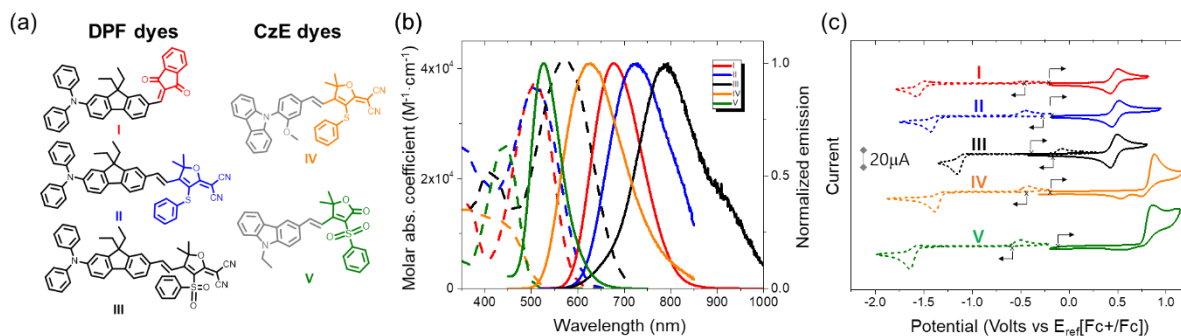
Figure 1. (a) Structures of dyes I-V . (b) Molar absorption coefficients (dashed) and normalized fluorescence (solid line) of dyes I (red), II (blue), III (black), IV (orange), and V (green) in \text{CHCl}_3 ( 2.5 \mu\text{M} ), excited at their absorption maximum. (c) Cyclic voltammograms of dyes I-V ( 1 \text{ mM} ) in degassed DCM solutions using tetrabutylammonium perchlorate as the electrolyte ( 0.1 \text{ M} ), glassy carbon as the working electrode, platinum as the counter electrode, \text{Ag}/\text{Ag}^+ as the reference electrode and a scan rate of 100 \text{ mV/s} .
