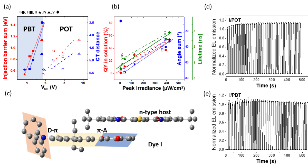
Figure 4. (a) Correlation between the device turn-on voltage ( V_{\text{on}} ) and the injection barrier sum (red) and CT distance (blue) for dye I (circle), II (square), III (star), IV (triangle) and V (diamond) in the /PBT (filled shaped) and /POT (open shapes) devices. (b) Correlation of the peak irradiance with the QY yield in solution (red) lifetime in solution (green) and the angle sum (blue, A_{\pi\text{D}} + A_{\pi\text{A}} ) for dye I (circle), II (square), III (star), IV (triangle) and V (diamond) in the /PBT (filled shaped) and /POT (open shapes) devices. (c) Optimized structures of I and BBOT showing the small A_{\pi\text{A}} and possible dye-host interactions on the acceptor side. (d) Stability of the I/POT devices upon 34 cycles of turn-on ( \sim 3 s) and turn-off ( \sim 3 s) driven by an average pulsed current of 11 \text{ mA/cm}^2 . (e) Stability of the I/PBT devices upon 41 cycles of turn-on ( \sim 3 s) and turn-off ( \sim 3 s) driven by an average pulsed current of 222 \text{ mA/cm}^2 .
