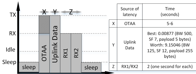
Figure 4: Medium access and latency source in LoRaWAN
