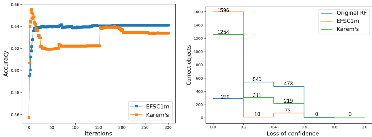
(a) Accuracy change in the iterative process (b) Correct objects in different intervals of loss of confidence
