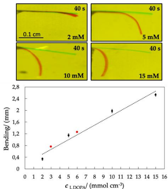
Figure 4. Concentration dependent deflection of Ppy for the enantioselective recognition of L-DOPA on oligo-(S)-BT2T4/Ppy. The readout time for each concentration is 40 sec. Length of the bipolar electrode is 1.1 cm. The electric field is 0.6 V/cm in all experiments. Error bars correspond to three repetitions. Red dots refer to Ppy deflection for chiral recognition of L-DOPA (3mM, 6mM, respectively) in the simultaneous presence of D-DOPA (6mM, 3mM, respectively).
