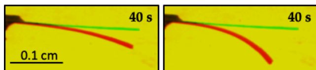
Figure 5. Enantioselective deflection of Ppy for two different solutions containing different ratios of L/D DOPA (3mM/ 6mM left, 6mM/ 3mM right). Oligo-(S)-BT2T4 was deposited on Ppy. The readout time for each concentration is 40 sec. Length of the bipolar electrode is 1.1 cm. The electric field is 0.6 V/cm in all the experiments.
