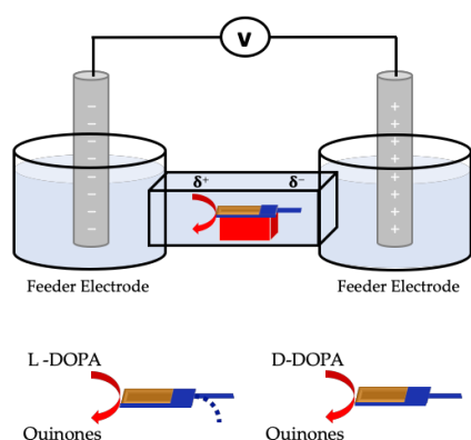
Scheme 2. Schematic illustration of the bipolar cell used for wireless absolute discrimination of D- and L-DOPA. The dark brown part stands for the (S)-BT2T4 oligomer, whereas blue symbolizes the Ppy film. The dotted blue line represents the Ppy bending after enantioselective recognition. The distance between feeder electrodes is 5 cm and the length of the bipolar electrode is 1.1 cm.
