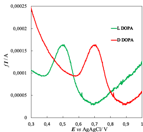
Figure 2. Differential pulse voltammetry in 0.2M LiClO 4 for the enantioselective electrooxidation of L- and D-DOPA (5 mM) on the surface at an oligo-(S)-BT2T4 surface, deposited on a free-standing Ppy film.
