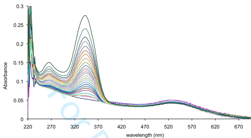
Figure S12: Evaluation of the UV-vis absorption spectrum of 1.Eu-AuNPs ( 1 \times 10^{-7} \text{M} ) in HEPES buffered solution (0.1M, ionic strength 0.1M NaCl) upon addition of nta 0-250 equivalents.
