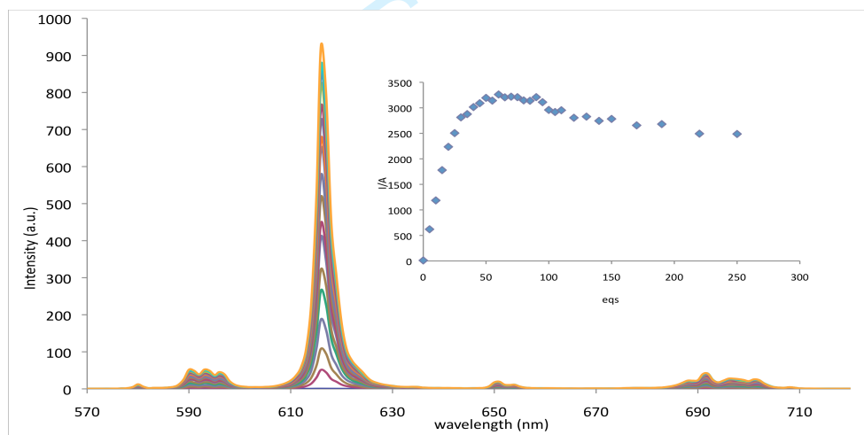
Figure S13: The changes in the \text{Ln}^{3+} centred emission of 1.Eu-AuNPs ( 1 \times 10^{-7} \text{M} ) in HEPES (0.1M, ionic strength 0.1M NaCl) upon the addition of nta 0-250 equivalents. Inset: The changes in the \text{Eu}^{3+} emission at 615 nm versus the number of equivalents of nta added.
