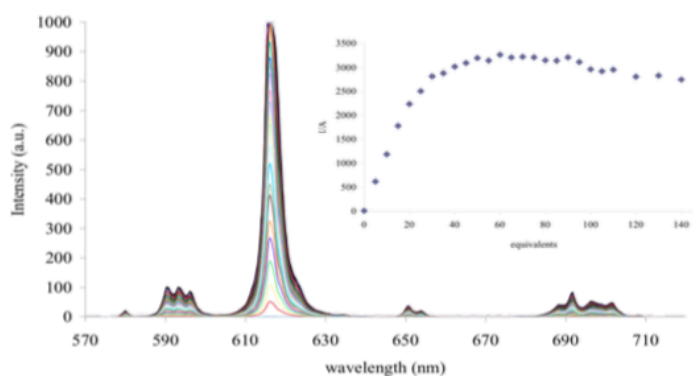
Figure S13: The changes in the \text{Ln}^{3+} centred emission of 1.Eu-AuNPs ( 1 \times 10^{-7} \text{M} ) in HEPES (0.1M, ionic strength 0.1M NaCl) upon the addition of nta 0-250 equivalents. Inset: The changes in the \text{Eu}^{3+} emission at 615 nm versus the number of equivalents of nta added.
