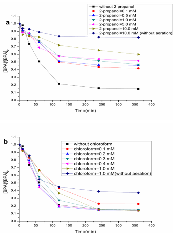
Fig. 5 BPA degradation in the modified photo-Fenton system in the presence of different scavenger a 2-propanol and b chloroform concentrations (conditions: [EDDS]=1.0 mmol L -1 , [ferrihydrite]=0.6 g L -1 , [H 2 O 2 ]=0.5 mmol L -1 , [BPA] 0 =20 μmol L -1 , pH=7).
