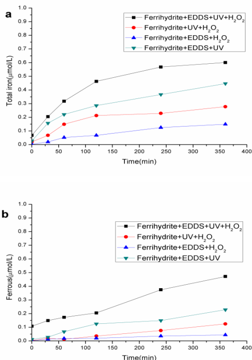
Fig. 6 a total iron dissolution rate and b ferrous dissolution rate in different systems (conditions: [EDDS]=1.0 mmol L -1 , [ferrihydrite]=0.6 g L -1 , [H 2 O 2 ]=0.5 mmol L -1 , [BPA] 0 =20 μmol L -1 , pH=7).
