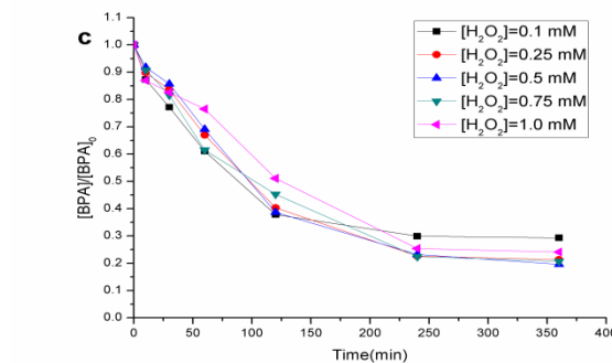
Fig. 3 Effects of BPA degradation in the modified photo-Fenton systems at a EDDS concentration (conditions: [ferrihydrate]=0.6 g L -1 , [H 2 O 2 ]=0.5 mmol L -1 , [BPA] 0 =20 μmol L -1 , pH=7), b ferrihydrate loading (conditions: [EDDS]=1.0 mmol L -1 , [H 2 O 2 ]=0.5 mmol L -1 , [BPA] 0 =20 μmol L -1 , pH=7), and c H 2 O 2 concentration ([EDDS]=1.0 mmol L -1 , [ferrihydrate]=0.6 g L -1 , [BPA] 0 =20 μmol L -1 , pH=7).
