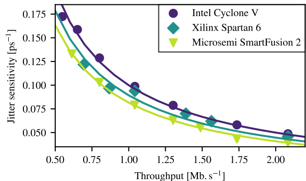
Fig. 3: Scatter plot and curve fit with a reciprocal function of the jitter sensitivity against the throughput for several PLL-TRNG configurations for each FPGA family
