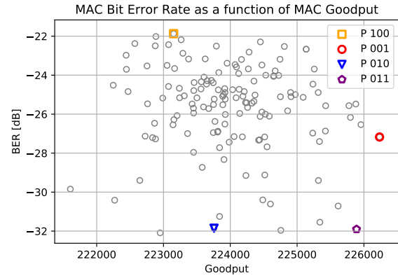
Fig. 4. Achievable BER at MAC layer as a function of the Goodput at PHY layer, varying the parameters of the probabilistic algorithm.
