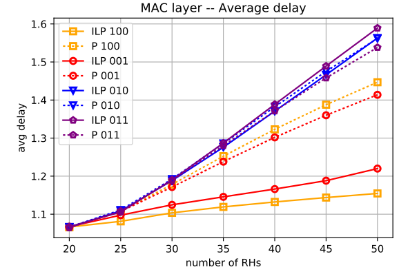
Fig. 2. MAC-layer performance of the scheduling algorithm via ILP.
