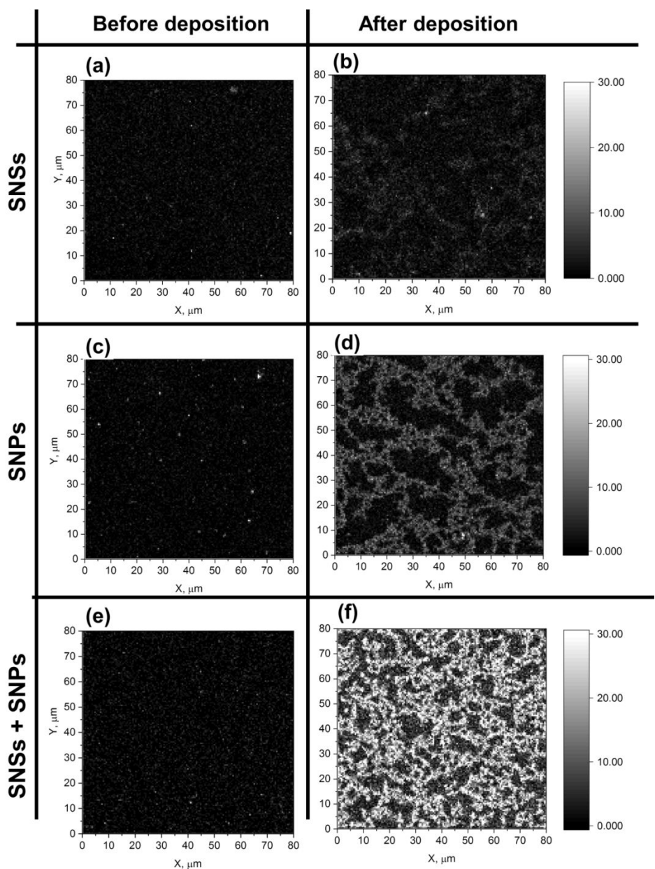
Figure 4. Confocal microscopy PL images of QD-in-PMMA films with a total thickness of 10 nm before (a, c, e) and after (b, d, f) deposition of PNPs: (a, b) before and after SNS deposition, (c, d) before and after SNP deposition, (e, f) before and after deposition of the mixture of SNSs and SNPs.
