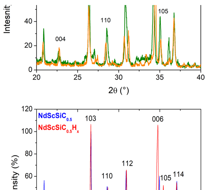
Figure 1. X-ray diffraction patterns for \text{NdScSiC}_{0.5} and \text{NdScSiC}_{0.5}\text{H}_x indexed with the space group I4/mmm .
