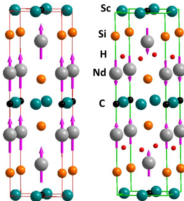
Figure 10. Magnetic structure of NdScSiC 0.5 (left) and NdScSiC 0.5 H 0.21 (right).
