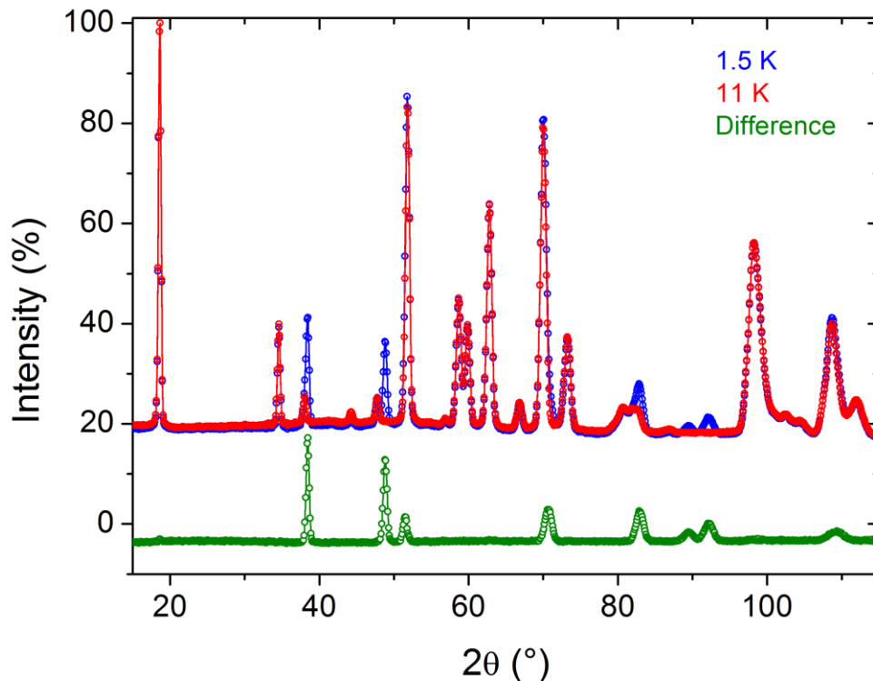
Figure 9. Neutron diffraction pattern of \text{NdScSiC}_{0.5}\text{H}_{0.21} at 11 and 1.5 K with the difference pattern plotted below to illustrate the magnetic peaks.
