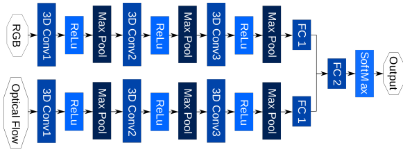
Figure 1: SSTCNN architecture
