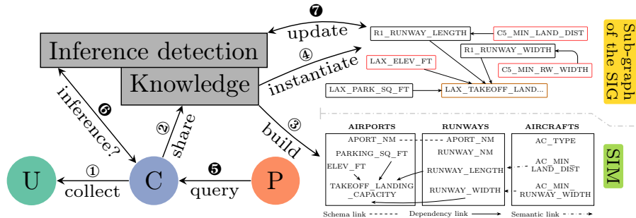
Figure 1: Workflow of the Chen et al. solution.
