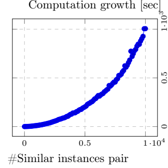
(b) GIG computation time growth.
