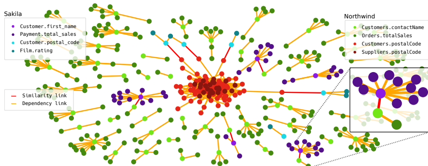
Figure 3: GIG with four pairs of similar customer instances.
