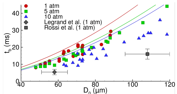
Figure 4: Measured burning time t_b with particle size D_0 and pressure as well as data from literature [10, 13]. Lines: Beckstead's correlation Eq. (1).
