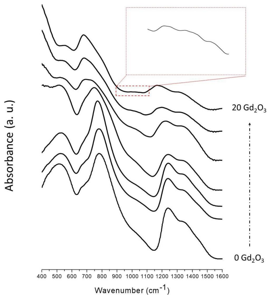
Fig. 8. Absorption spectra in the infrared range for samples with concentrations of Gd 2 O 3 from 0 to 20 mol%. The red dashed box is a magnification in the selected area of the spectrum for the sample with 20 mol% of Gd 2 O 3 to evidence the rise of three low-intensity peaks. (For interpretation of the references to color in this figure legend, the reader is referred to the Web version of this article.)
