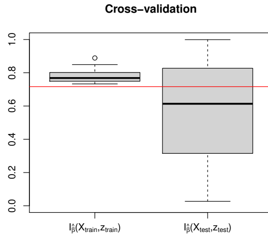
Figure 7: Boxplot of I_{\hat{\beta}_{train}}(X_{test}, Z_{test}) . The red line represents I_{\hat{\beta}}(X, Z) computed from all the observations.
