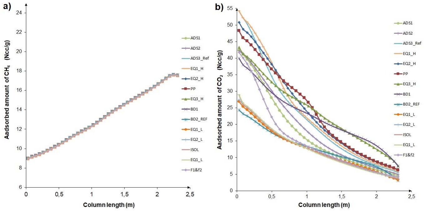
Figure 13 Adsorbed amount of CH 4 and CO 2 at the end of each step as a function of the axial position with 60% recycling and P des =0.1 bara a) CH 4 adsorbed amount with 60% recycling, b) CO 2 adsorbed amount with 60% recycling
