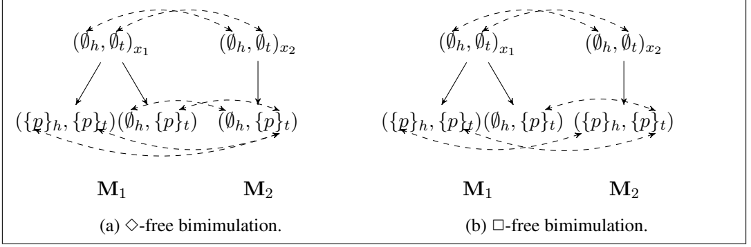
Figure 2: \Diamond -free and \Box -free bimimulations.
