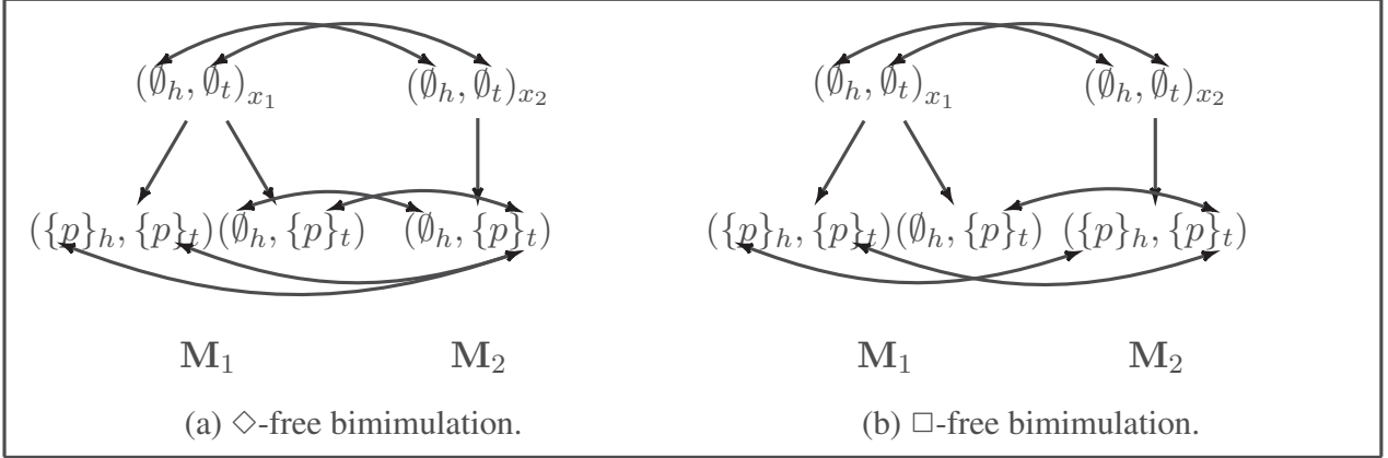
Figure 2: \diamond -free and \square -free bimimulations.
