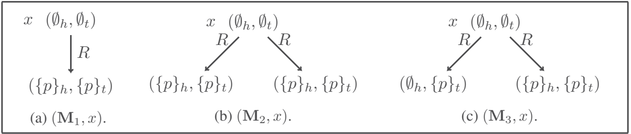
Figure 3: Three KHT pointed models satisfying \diamond p .
