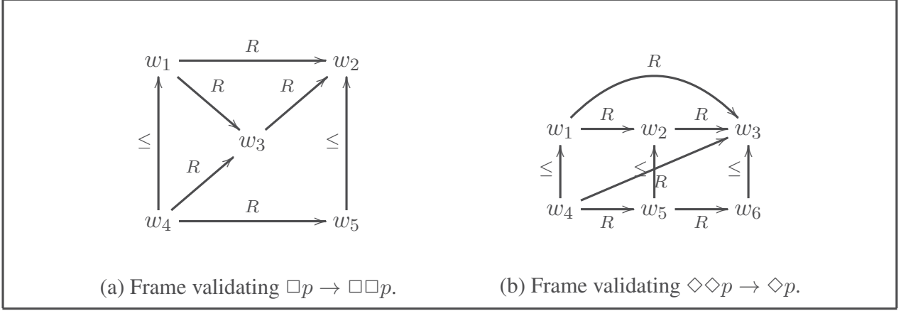
Figure 1: Non-transitive and strongly normal frames
