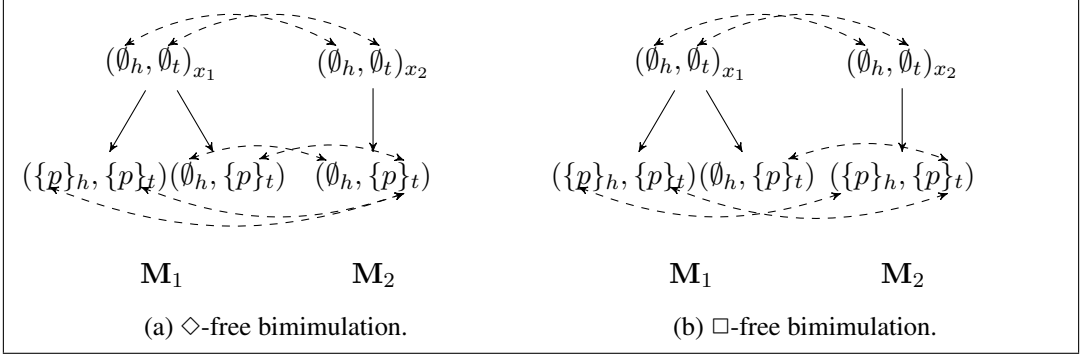
Figure 2: \diamond -free and \square -free bimimulations.
