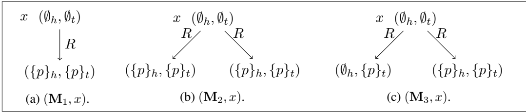
Figure 3: Three KHT pointed models satisfying \diamond p .
