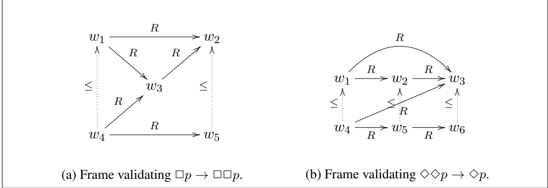
Figure 1: Non-transitive and strongly normal frames
