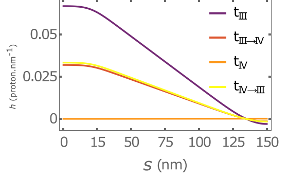
FIG. 3. Dynamics of the proton field along the cristae. The plots represent the field h(s, t) solution of Eq. (3) for parameter values given in Table I and for t_{\text{IV}} = 0 [T] , t_{\text{IV} \rightarrow \text{III}} = T/4 [T] , t_{\text{III}} = T/2 [T] , t_{\text{III} \rightarrow \text{IV}} = 3T/4 [T] . The concentration h(s, t) is expressed in proton per nm.
