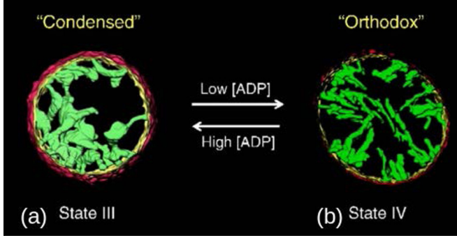
FIG. 1. Cross section of a mitochondrion in different states of ATP production [2]. (a) State III, for which sugar in excess is available leading to a high rate of ATP production. (b) State IV, for which no sugar is available leading to a vanishing ATP production rate. Mitochondria (left to right) have diameters of 1500 nm and 500 nm.
