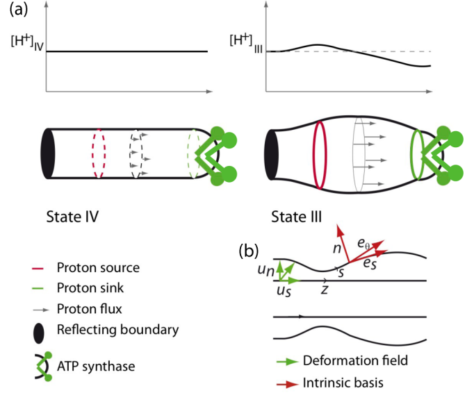
FIG. 2. Schematic representation of a crista. (a) The plots represent the proton concentration on the surface in states III and IV. The tubes represent the shape of the invagination in state III and IV. (b) Deformation fields of the membrane and intrinsic basis of the deformed surface.
