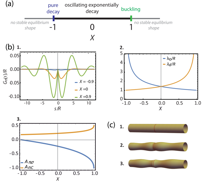
FIG. 4. (a) Stability diagram of a Helfrich cylinder as a function of X = C_{00}R . (b) 1. G_n(s)/R , Normalized Green functions for different values of X = -0.9, 0, 0.9 and for \delta\sigma = 0.15 and \delta C_0 = 0 . 2. Characteristic lengths of oscillation \lambda_0 and decay \lambda_d as a function of X . 3. Maximal amplitude of the deformations driven respectively by a variation of \sigma , A_{n\sigma} and by a variation of C_0 , A_{nC} . (c) Three-dimensional representations of a cylinder (top) deformed by h(s) = \delta(s) for ( X = 0.96 , \delta\sigma = 0.2 , \delta\kappa = 0 , \delta C_0 = 0 ) (middle), and for ( X = 0.96 , \delta\sigma = -0.2 , \delta\kappa = 0 , \delta C_0 = 0 ) (bottom). All quantities are dimensionless.
