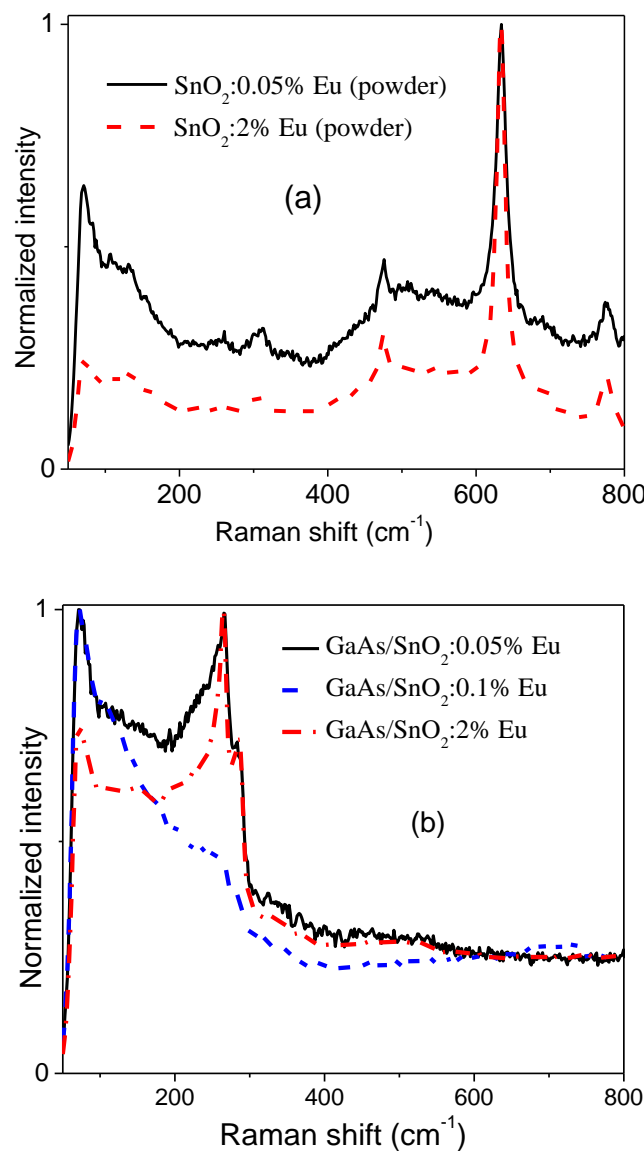
Fig. 6. (a) Raman spectra of \text{SnO}_2:0.05\% \text{ Eu} and \text{SnO}_2:2\% \text{ Eu} powders. (b) Raman spectra of \text{GaAs/SnO}_2:0.05\% \text{ Eu} , \text{GaAs/SnO}_2:0.1\% \text{ Eu} and \text{GaAs/SnO}_2:2\% \text{ Eu} heterostructures.
