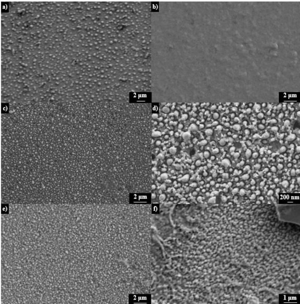
Fig 1. Surface images for: (a) GaAs thin film (FESEM- scale bar: 2 \mu\text{m} ), (b) SnO 2 :2%Eu thin film (SEM- scale bar: 2 \mu\text{m} ); (c) heterostructure GaAs/SnO 2 :2%Eu annealed at 200°C/1 hour (SEM- scale bar : 2 \mu\text{m} ) (d) GaAs/SnO 2 :2%Eu annealed at 200°C/1 hour (FESEM- scale bar: 200 nm) (e) GaAs/SnO 2 :2%Eu annealed at 400°C/20 min (SEM- scale bar: 2 \mu\text{m} ). (f) GaAs/SnO 2 :2%Eu annealed at 400°C/20 min (FESEM- scale bar: 1 \mu\text{m} ).
