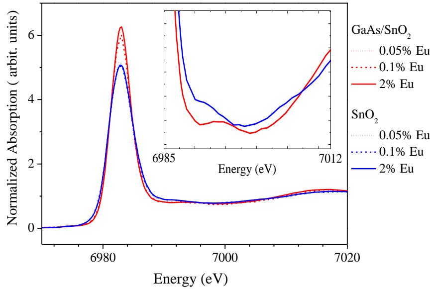
Fig. 2. XANES comparison between GaAs/SnO 2 :Eu heterostructures and SnO 2 :Eu films. The white line is found at the same value (6982.8 eV). Inset: Differences are very clear in the secondary's structures just above the absorption edge energy.
