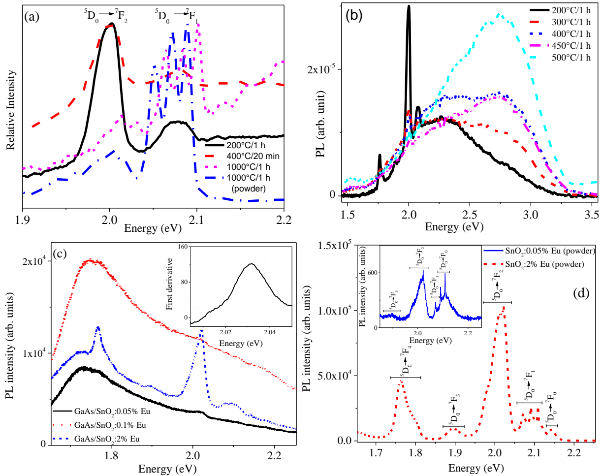
Fig.5. (a) PL relative intensity with magnification of {}^5\text{D}_0 \rightarrow {}^7\text{F}_1 and {}^5\text{D}_0 \rightarrow {}^7\text{F}_2 emission peaks of GaAs/ \text{SnO}_2:2\%\text{Eu} heterostructure thermally annealed at 200^\circ\text{C} and at 400^\circ\text{C} and \text{SnO}_2:2\%\text{Eu} film and powder with thermal annealing of 1000^\circ\text{C} . (b) PL of heterostructure with distinct thermal annealing: 200, 300, 400, 450 and 500^\circ\text{C} by 1 h. (c) PL for GaAs/ \text{SnO}_2:0.05\%\text{Eu} and GaAs/ \text{SnO}_2:0.1\%\text{Eu} annealed at 200^\circ\text{C} and GaAs/ \text{SnO}_2:2\%\text{Eu} annealed at 400^\circ\text{C} by 20 min. Inset: First derivative curves of GaAs/ \text{SnO}_2:0.05\%\text{Eu} and GaAs/ \text{SnO}_2:0.1\%\text{Eu} . (d) PL for \text{SnO}_2:2\%\text{Eu} powder. Inset: PL for \text{SnO}_2:0.05\%\text{Eu} powder. Excitation: (a) and (b): line 350 nm of the \text{Kr}^+ laser, (c) and (d): line 488 nm of the \text{Ar}^+ laser.
