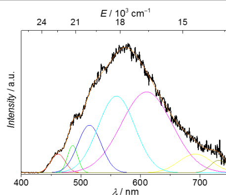
Figure 3 Phosphorescence spectrum of the Gd-1 MC measured in the solid state under excitation at 325 nm (77 K, 100 \mu s delay after the excitation flash, black trace) and its Gaussian decomposition (colored traces).
