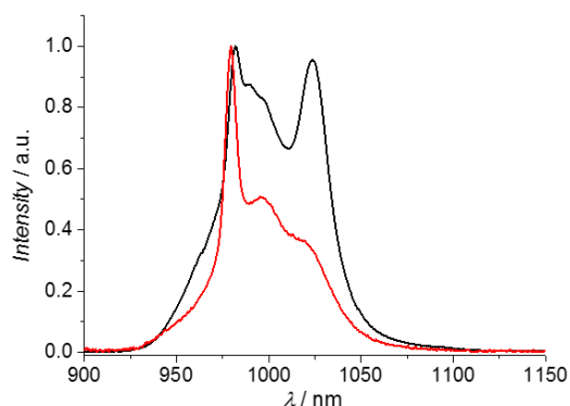
Figure 6 Corrected and normalized emission spectra of the Yb-1 MC collected in the solid state ( \lambda_{ex} = 350 nm, black trace) and in methanol solutions ( \lambda_{ex} = 320 nm, 0.5 mM, red trace) at room temperature.
