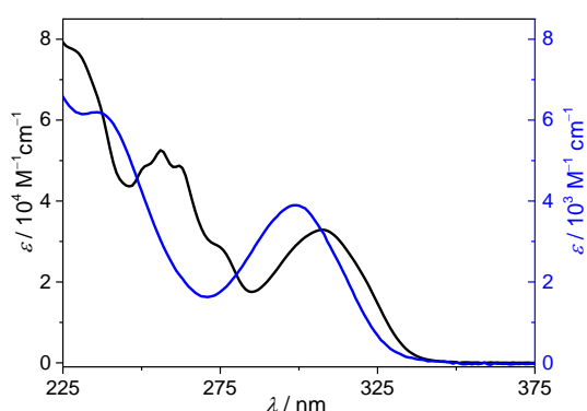
Figure 2 Absorption spectra of the Gd-1 MC recorded in CH 3 OH solutions (black trace, left scale) and H 3 shi (blue trace, right scale).
