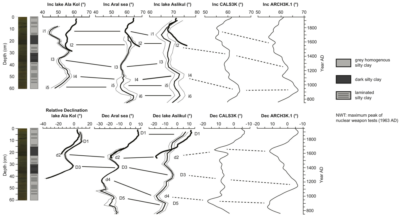
Fig. 4. Paleomagnetic secular variations (PSV). Paleomagnetic data have been plotted as mean values of 40-year intervals, and contours of 95% circles of confidence. Thick black lines for inclination and declination data correspond to historical observations of the magnetic field between 1590 and 1990 CE modelled for the three localities (Lake Ala Kol, Aral Sea, Lake Aslikul). PSV data from Lake Ala Kol (plotted versus depth) are compared with natural archives from Aral Sea (Nourgaliev et al., 2003) and Lake Aslikul (Nourgaliev et al., 1996, 2000), the spherical harmonic GUFM1 model (Jackson et al., 2000), the ARCH3k.1 and CALSK3k.4 models (Korte et al., 2009, 2011). The GUFM1, ARCH3k.1 CALSK3k.4 curves were modelled for our site location (N42°19'03.7"; E78°32'59.5"). All reference curves are plotted versus age. Note that PSV data rely exclusively on ChRM inclination and relative declination data (no relative paleointensity, see text for detail).
