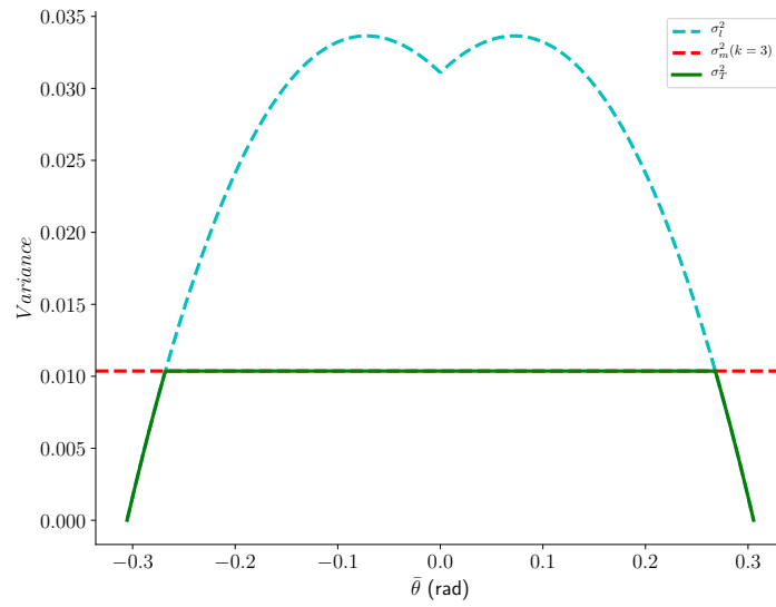
Figure 9. Thresholds \sigma_I , \sigma_m and \sigma_T relative to \hat{\theta} with b = 0.61 radians (35 deg).
