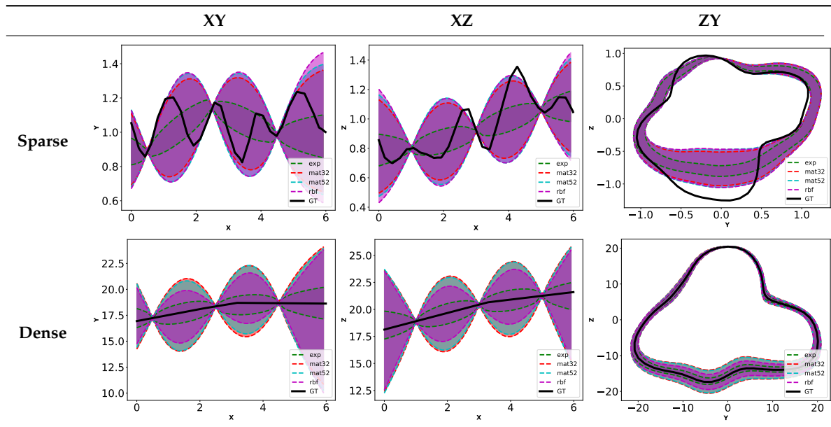
(b) Learned lengthscale l_\psi (values in Table 2).
