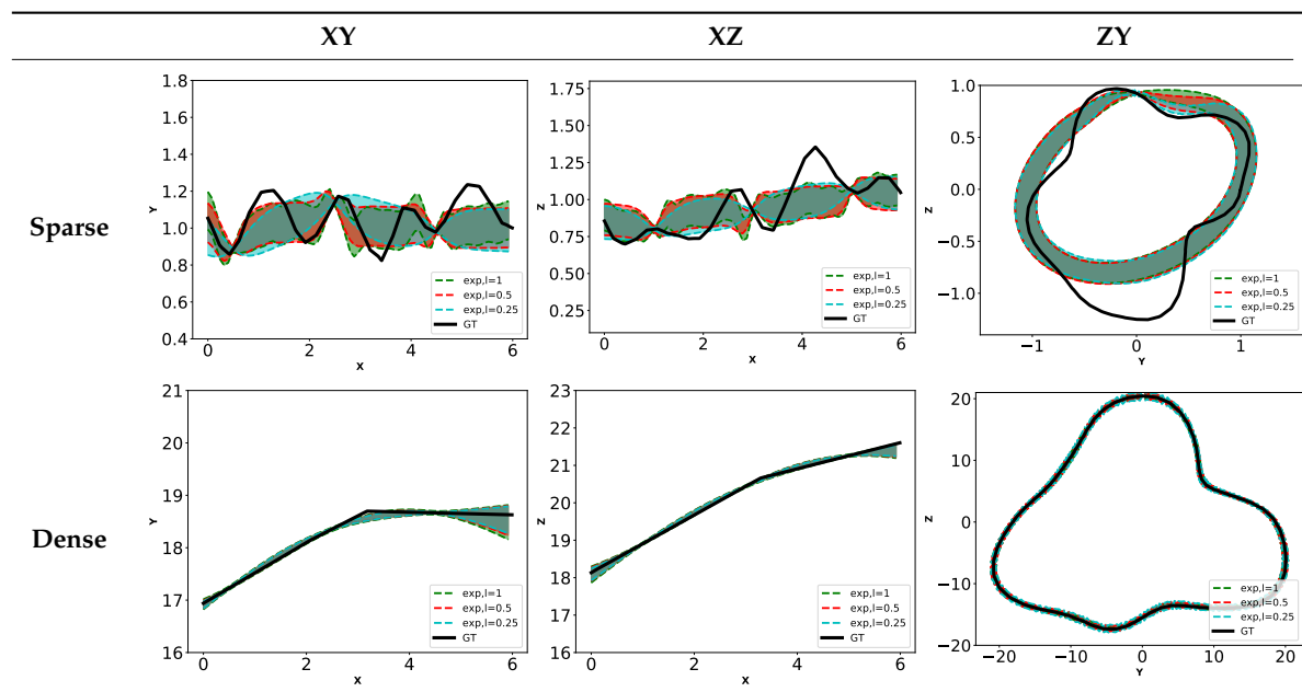
(a) K_\psi = K^{exp} \circ d_{chordal}
