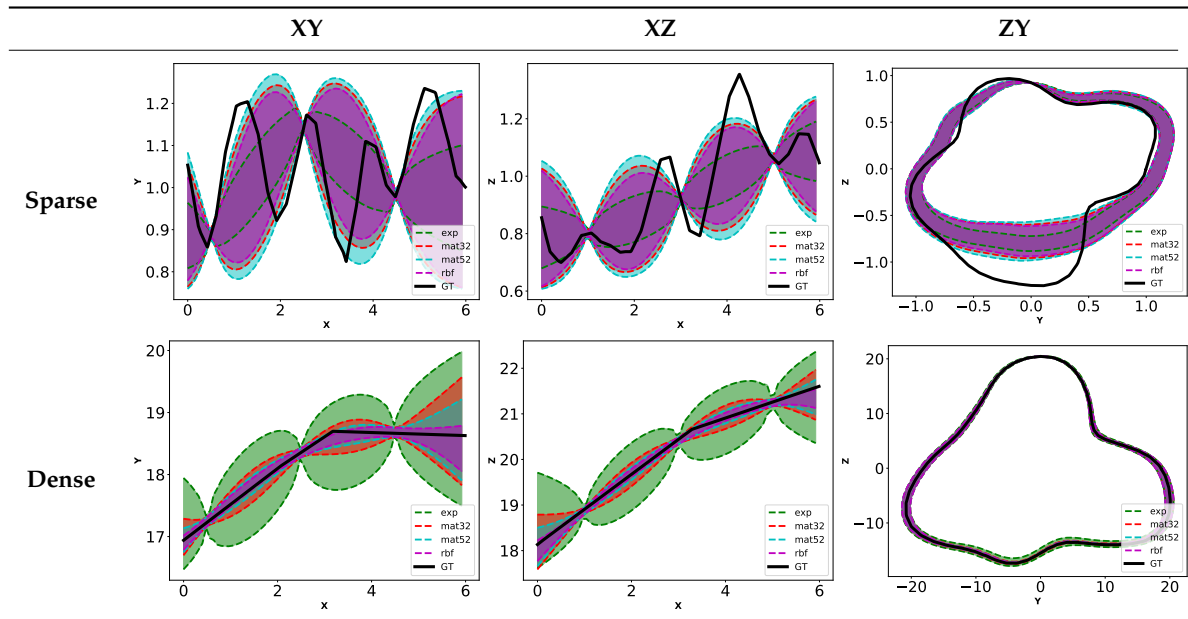
(a) Fixed Lengthscale l_\psi = 0.5 .
