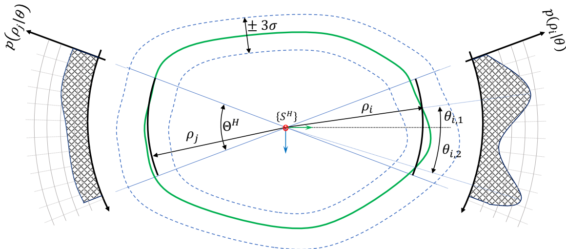
Figure 6. Illustration of elevation angle maximum likelihood estimation on a vertical slice. The green curve is the mean surface (cofounded here with the true surface for visibility) and blue curves are the confidence interval at \pm 3\sigma . Note that in this particular configuration \rho = \rho^h = \hat{\rho}^v .
