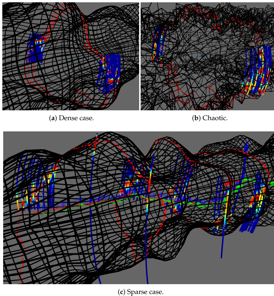
Figure 17. Distributions obtained in the experiment with K_s = K_{\text{sur}}^M . For better visibility, uniform distributions are not displayed.
