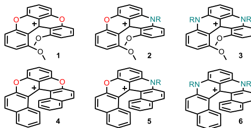
Figure 1. Dioxa, azaoxa and diaza [4] and [6]helicenes 1-6 .
