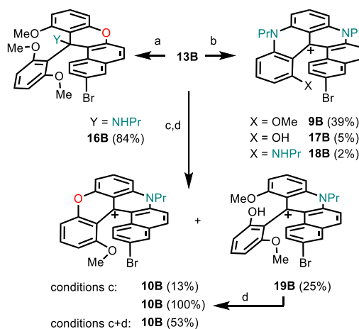
Scheme 2. Synthesis of azaoxa and diaza [5]helicenes 9B and 10B and solid state structure of 16B.
