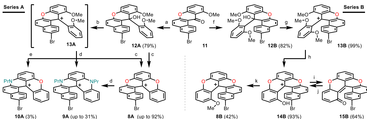
Scheme 1. Synthesis of a series of bromo-substituted [5]helicenes.
