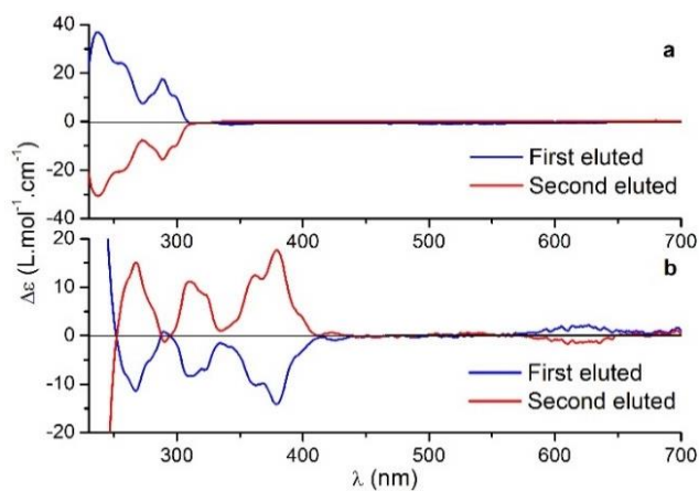
Figure 4. ECD spectra of compounds derived from the first and second eluted enantiomers of: a) reduced dioxa 23A ; b) cationic
