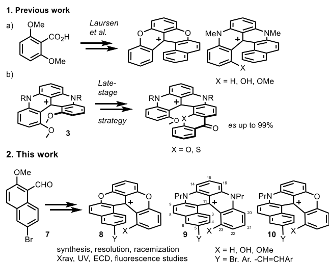
Figure 2. Synthesis of cationic [5]helicenes. The numbering of key helicene positions are indicated on compound 9 .
