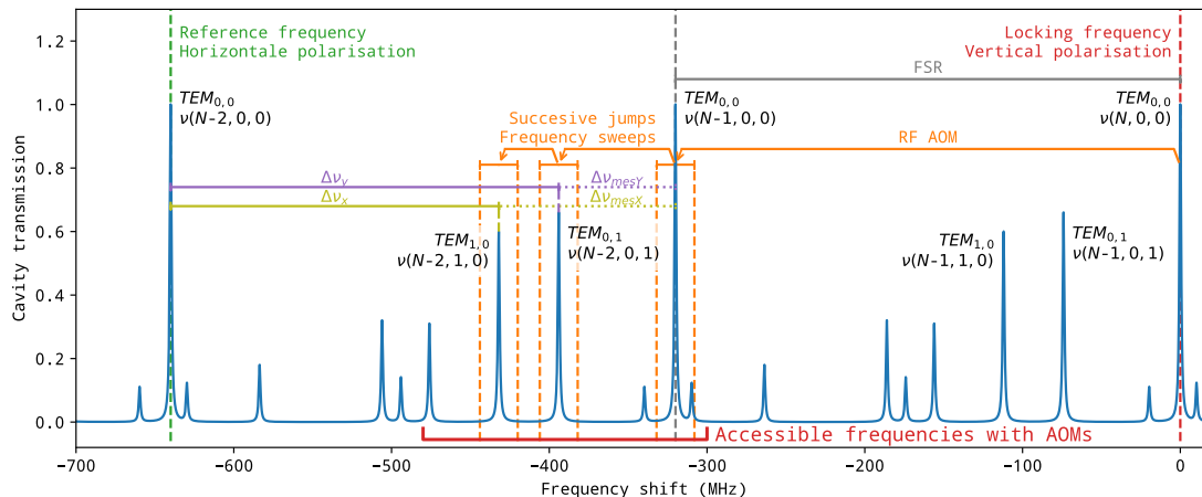
Figure 4: Measurement of \Delta\nu values. AOMs RF range limitations impose to evaluate the frequency intervals relative to the end of the mode structure ( \Delta\nu_{mess} quantities). From there, the \Delta\nu quantities are deduced using evaluation of FSR (in gray).
