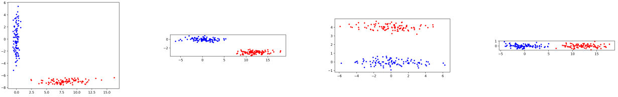
Figure 1 – Considered illustrative 2D data sets, from left to right \mathcal{D}_1 , \mathcal{D}_2 , \mathcal{D}_3 , \mathcal{D}_4 ,
