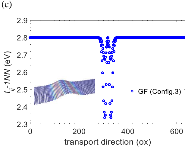
Fig. 6: Gaussian folds (GF): (a) T_e as a function of energy for several GF configurations in the ribbon of width M = 41 ( W_R \approx 49.19 \text{ \AA} ), and length N = 150 ( L \approx 637.58 \text{ \AA} ). (b) Correlation between T_e (at E = 0 ) and the ratio h_G W_G / W_R . (c) & (d) Hopping profiles in the ribbon with the GF Configs. 3 & 4 presented in Fig. 6(a). Inset in Fig. 6(b) presents the cut-off ratio h_G W_G / W_R at T_e = 0.03 as a function of strain for different ribbon widths. Inset in Fig. 6(c) is the bonding map of the GF Config. 3, the color bar is from 1.42 \text{ \AA} to 1.5 \text{ \AA} as in Fig. 4.
