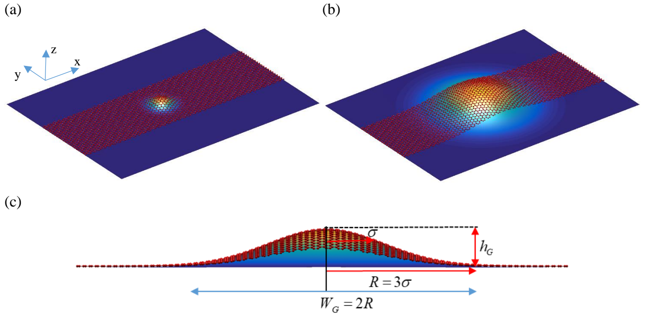
Fig 1: Sketch of a ribbon with Gaussian deformation. Two typical deformations are illustrated: (a) small and (b) large Gaussian bumps. (c) Parameters defining the shape of a Gaussian bump.
