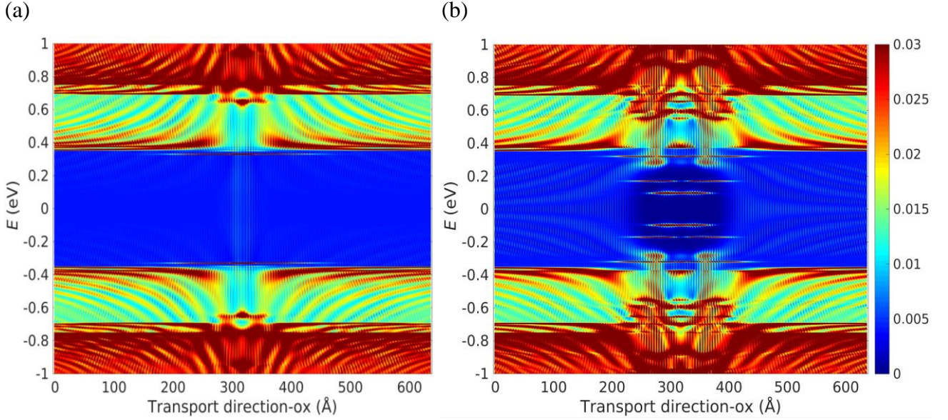
Fig. 3: LDOS (in arb. unit) as a function of energy and transport direction (ox) for two deformations: h_G = 6.67 \text{ \AA} , \sigma = 12.33 \text{ \AA} (Config. 3) and h_G = 25.27 \text{ \AA} , \sigma = 46.15 \text{ \AA} (Config. 4). M = 41 ( W_R \approx 49.19 \text{ \AA} ), N = 150 ( L \approx 637.58 \text{ \AA} ).
