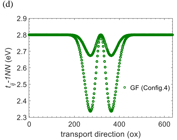
Fig. 6: Gaussian folds (GF): (a) T_e as a function of energy for several GF configurations in the ribbon of width M = 41 ( W_R \approx 49.19 \text{ \AA} ), and length N = 150 ( L \approx 637.58 \text{ \AA} ). (b) Correlation between T_e (at E = 0 ) and the ratio h_G W_G / W_R . (c) & (d) Hopping profiles in the ribbon with the GF Configs. 3 & 4 presented in Fig. 6(a). Inset in Fig. 6(b) presents the cut-off ratio h_G W_G / W_R at T_e = 0.03 as a function of strain for different ribbon widths. Inset in Fig. 6(c) is the bonding map of the GF Config. 3, the color bar is from 1.42 \text{ \AA} to 1.5 \text{ \AA} as in Fig. 4.
