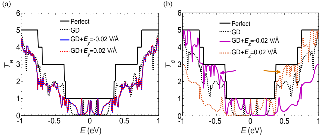
Fig. 9: An AGNR of width M = 41 ( W_R \approx 49.19 Å) and length N = 150 ( L \approx 637.58 Å) with a large Gaussian deformation (GD) h_G = 25.27 Å, \sigma = 46.15 Å under the effect of (a) a transverse electric field \vec{E} = E_y \cdot \vec{e}_y and (b) a vertical electric field \vec{E} = E_z \cdot \vec{e}_z .
