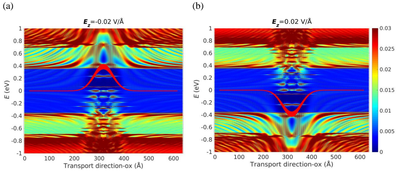
Fig. 10: LDOS versus E -ox for opposite fields (a) \mathbf{E}_z = -0.02 \text{ V/\AA} and (b) \mathbf{E}_z = 0.02 \text{ V/\AA} . Red lines are electrostatic potential profiles induced by the electric fields. Here M = 41 ( W_R \approx 49.19 \text{ \AA} ), N = 150 ( L \approx 637.58 \text{ \AA} ) and the Gaussian bump h_G = 21.36 \text{ \AA} , \sigma = 39.01 \text{ \AA} . In both panels, LDOS is in arb. unit.
