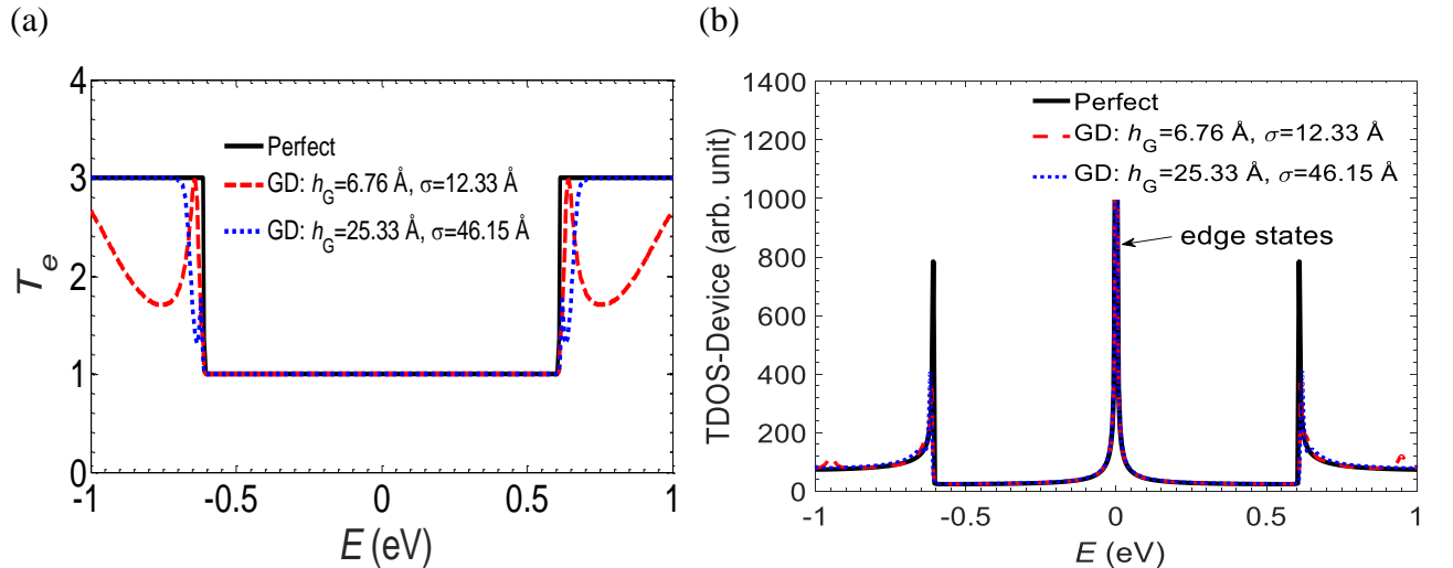
Fig. 8: (a) Transmission and (b) TDOS of a device made of a ZGNR of width M = 20 ( W_R \approx 41.18 \text{ \AA} ), N = 150 ( L \approx 367.69 \text{ \AA} ).
