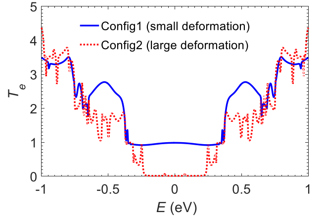
Fig. 14: (a) Illustration of an imperfect Gaussian deformation made by a mixing of two close Gaussian bumps, one is at the ribbon center and the other is off-center at V_{\text{off}} = (x_0/15, y_0/15, 0) . The color gradient presents the height of atoms. (b) Electron transmission of two configurations of deformation: small (Config1): h_{G1} = 5.48 \text{ \AA} , \sigma_1 = 10 \text{ \AA} ; h_{G2} = 5.59 \text{ \AA} , \sigma_2 = 11 \text{ \AA} and large (Config2): h_{G1} = 27.39 \text{ \AA} , \sigma_1 = 50 \text{ \AA} ; h_{G2} = 27.66 \text{ \AA} , \sigma_2 = 51 \text{ \AA} .
