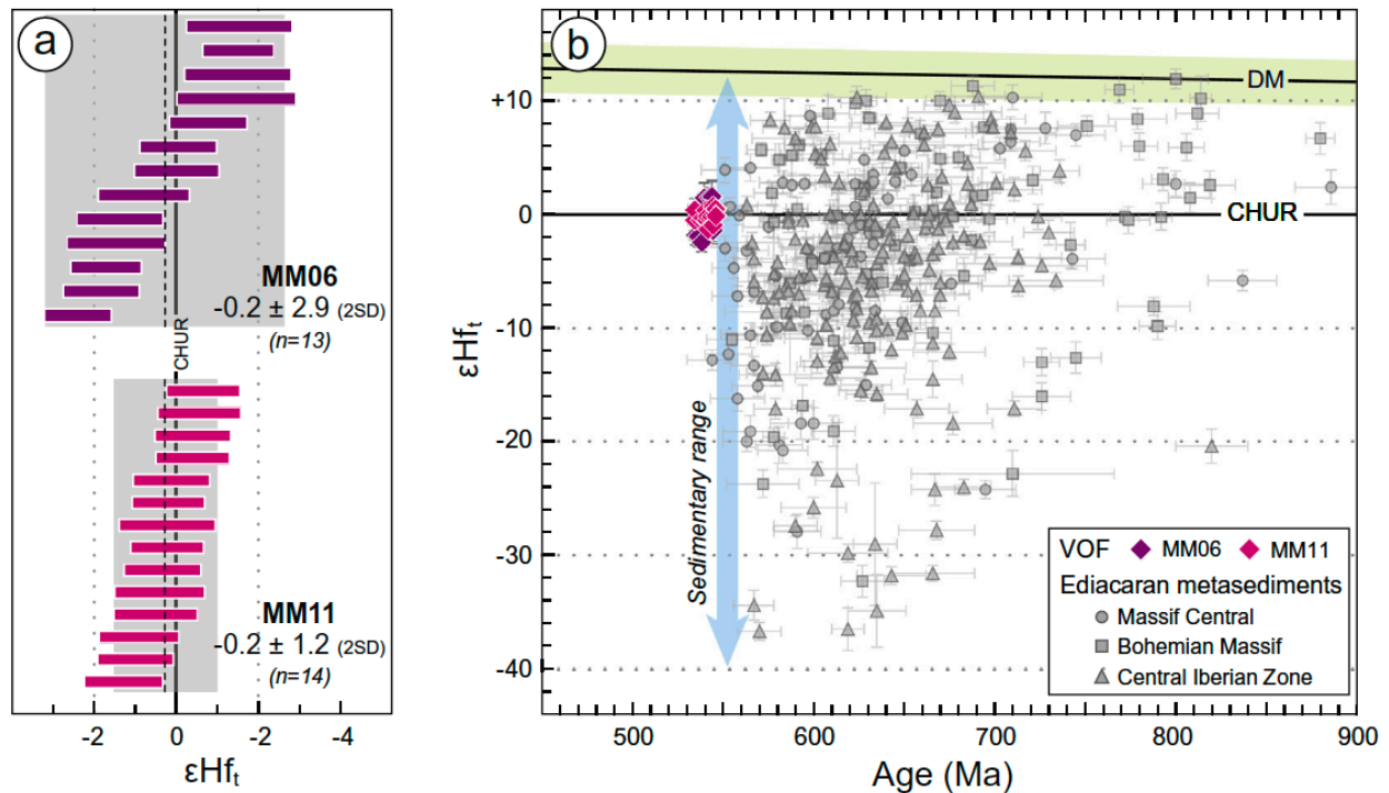
Figure 9: (a) Measured \epsilon\text{Hf}(t) on magmatic zircon grains and rims from the two investigated samples of augen gneisses of the Velay Orthogneiss Formation (VOF). (b) Zircon \epsilon\text{Hf}(t) vs. age diagram for the two VOF samples and a compilation of data from detrital zircon in regional Ediacaran metasediments ( n=371 ), regarded as the potential source of the peraluminous magmas from which the VOF protoliths derive. Data from the French Massif Central (Chelle-Michou et al., 2017), the Bohemian Massif (Linnemann et al., 2014) and the Iberian Massif (Orejana et al., 2015; Teixeira et al., 2011). The \epsilon\text{Hf}(t) range for the depleted mantle reservoir is bracketed by the models of Naeraa et al. (2012) (lowermost value) and Griffin et al. (2002) (uppermost value).
