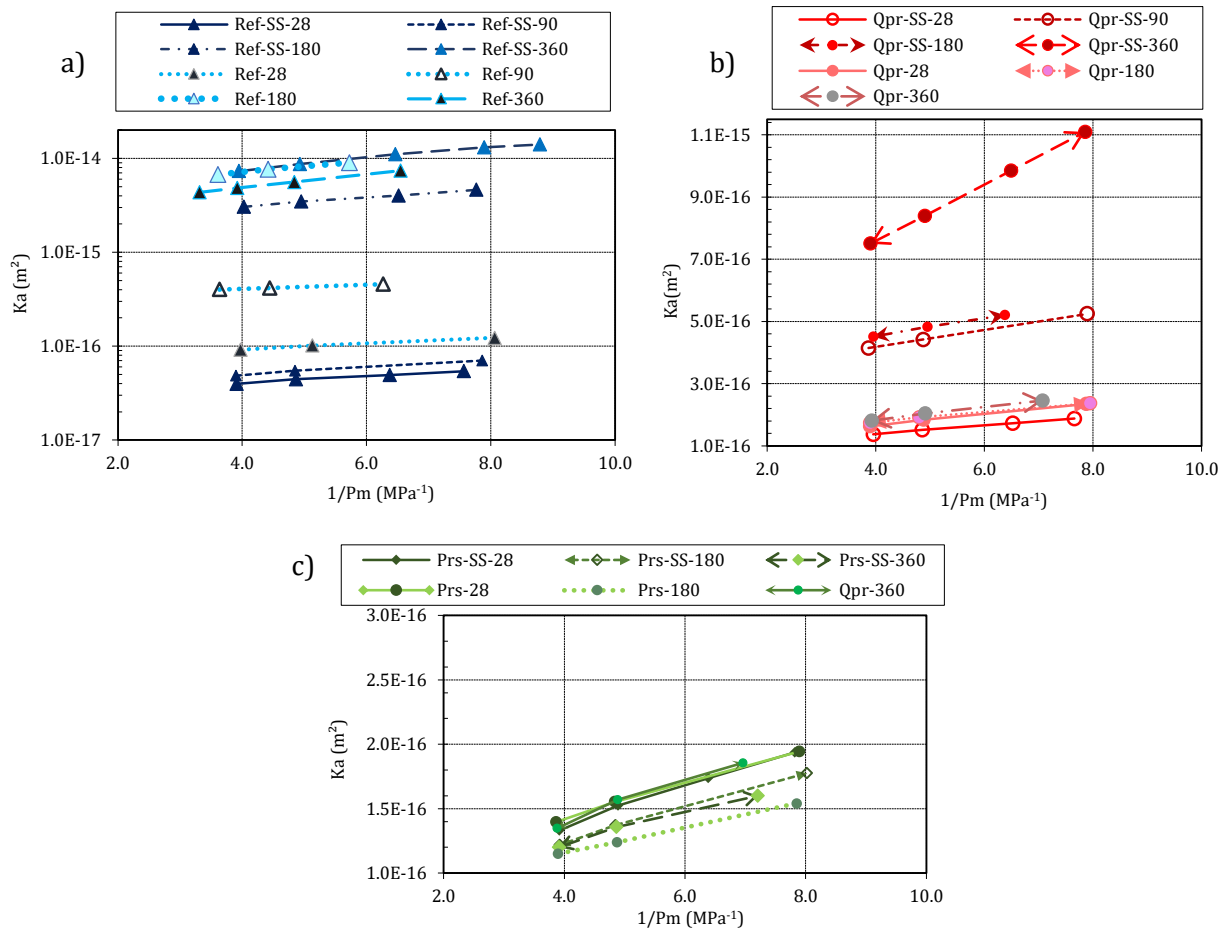
Figure 14– Apparent permeability at different ages for the mortars : “Ref-SS” (a) , “Ref” (a) , “Qpr-SS” (b), “Qpr” (b), “Prs-SS” (c) and “Prs” (c).
