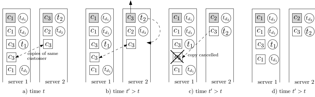
Figure 3: A two-server model with dedicated and flexible customers and \gamma_1 = \gamma_2 = 1 . All dedicated customers have a token, and only the first flexible customer in each queue has a token. The servers serve the queues in a FCFS fashion, so only the first (shaded) customer in the queue gets service. Part a) shows a snapshot of the system at some arbitrary time t . The second flexible customer of type c_3 has redundant copies in both servers, as it has not claimed token of classes t_1 or t_2 yet. Part b) shows the system at a time t' > t , when the first customer from server 2 departs. Because of this, the next customer in line, which is a dedicated customer, starts being served, the flexible customer in server 1 obtains a token and its redundant copy in server 1 is cancelled (part c)). Part d) shows the final configuration.
