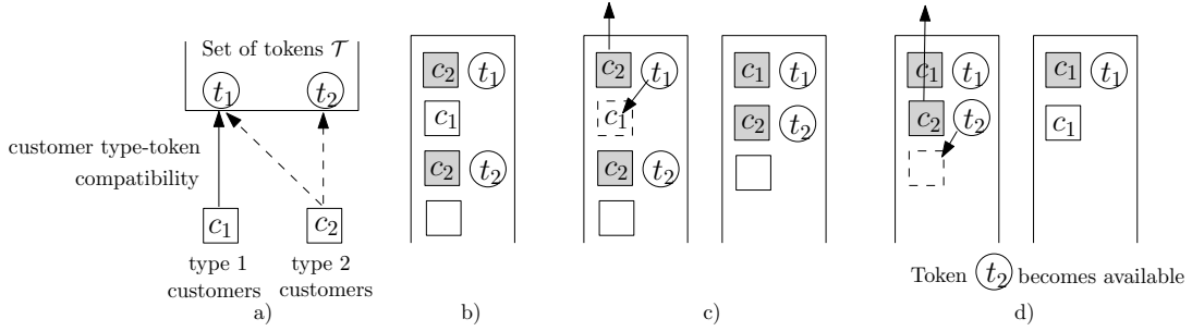
Figure 1: An example of a token-based model with token set \mathcal{T} = \{t_1, t_2\} . Grey-shaded customers are paired with tokens and can thus receive service. Figure b) depicts the initial state. Figure c) then sketches what happens when the first customer would leave: token t_1 scans the queue for the next compatible customer, and is then claimed by the oldest compatible customer, which is of type c_1 . Figure d) describes what happens if the customer holding token t_2 would then leave the system. Token t_2 again scans the rest of the queue for compatible customers, but it turns out that the last customer is of type c_1 , and token t_2 becomes available.
