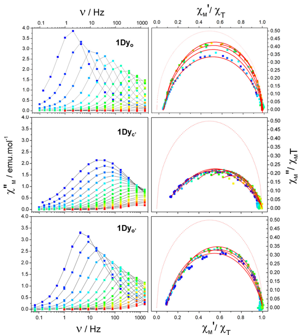
Figure 7. (left) Frequency dependence of the out-of-phase magnetic susceptibility \chi'' of 1Dy o , 1Dy c and 1Dy o' (from top to bottom) measured with a static magnetic field H_{\text{dc}} = 1200 \text{ Oe} between 2 K (blue) and 10 K (red). (right) Corresponding Cole-Cole plots with some of the best fits as red full lines and ideal relaxation curve ( \alpha = 0 , RF = 100%) as red dotted line.
