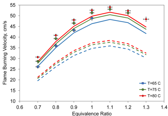
Fig. 3. Laminar burning velocity of mhx3d /air mixtures (at different unburnt gas temperature T ) as a function of equivalence ratio. Symbols: experiment, lines: modeling (dashed lines: original mechanism proposed by Zhang et al. [21], solid lines: updated mechanism).
