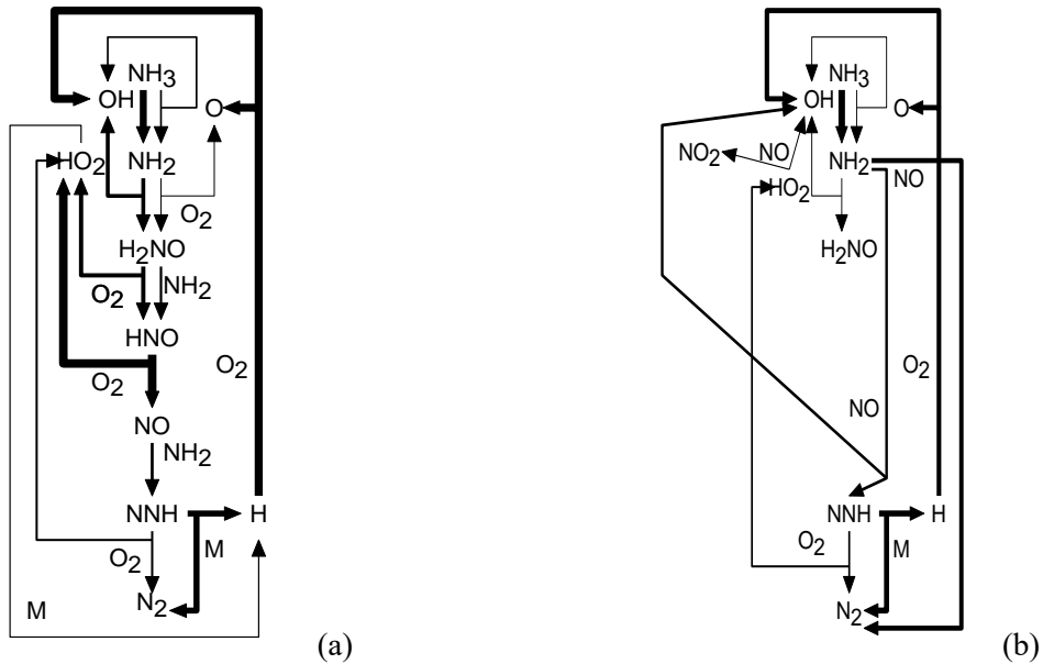
Figure 11. Computed reaction pathways for the oxidation of \text{NH}_3 in a JSR using the updated DGA model. (a): 1000 ppm of \text{NH}_3 , 12500 ppm of \text{O}_2 , \tau=100\text{ms} ; \phi=0.1 ; (b): 1000 ppm of \text{NH}_3 and 500 ppm of \text{NO} , \tau=100\text{ms} ; \phi=0.1 .
