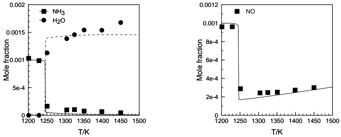
Figure 10. Comparison between experimental (symbols) and computed (lines) results for the oxidation of \text{NH}_3 in a JSR: 1000 ppm of \text{NH}_3 , 625 ppm of \text{O}_2 , and 1000 ppm of \text{NO} , \tau=200\text{ms} ; \phi=2 .
