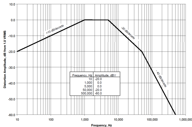
Figure 2. Profile of harmonic limits for avionics, DC bus 28Vdc (for the 270Vdc bus limits are 10 dB higher) [23].
