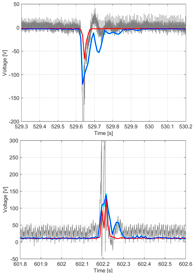
Figure 3. RMS of the bandpass ( f_1 - f_2 ) Butterworth (order 8) ripple index for 5-1000 Hz (cyan), 5-5000 Hz (blue) and 50-10000 Hz (red) (negative rms is for display purposes).
