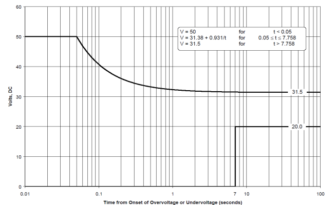
Figure 1. Profile of allowed transient overvoltage / undervoltage for avionics with DC bus 28Vdc [23].
