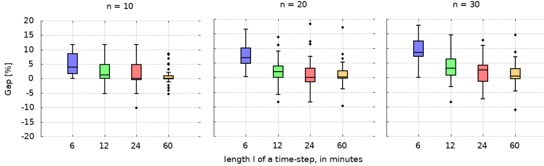
Figure 5: Distribution of gap(T^{D_{100}S720}, T^{D_{100}S^l}) with l \in \{6, 12, 24, 60\} for Problem P_1 .
