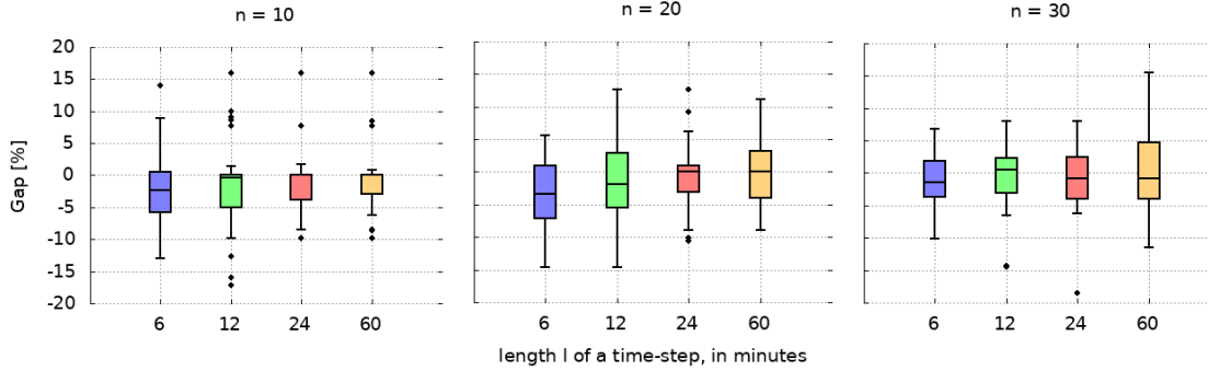
Figure 6: Distribution of gap(T^{D_{Lyon}S720}, T^{D_{Lyon}S^l}) with l \in \{6, 12, 24, 60\} for Problem P_1 .
