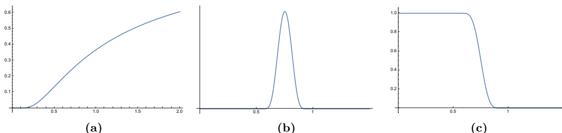
Figure 3. (a) Function X_0(t) for r = 1 ; (b,c) The corresponding functions X_1(t) and X(t) .
