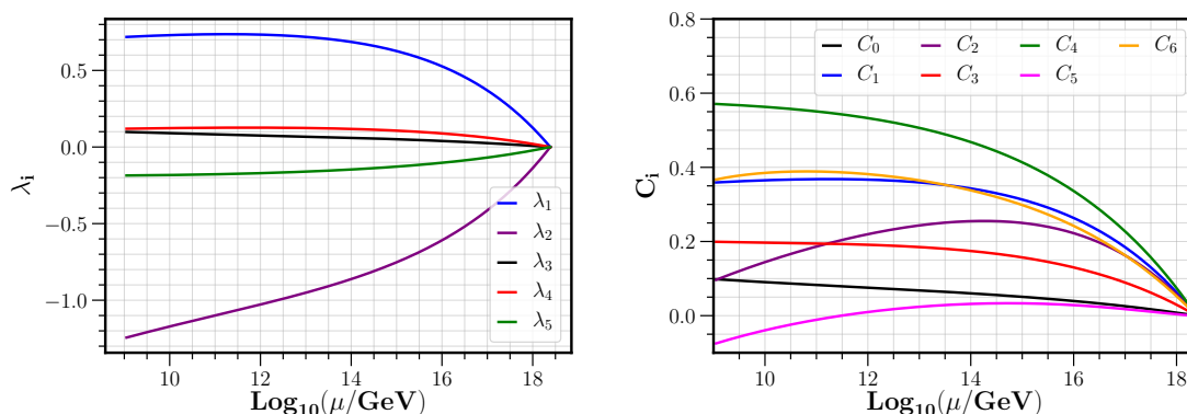
Figure 6. Running of the triplet quartic couplings (left figure) and the conditions for the classical stability of the potential (right figure) for M_\Delta = 10^9 \text{GeV} and Y_\Delta = 1.3 considering right-handed neutrinos with Y_\Phi = 0.37 . Left: all quartic couplings vanish at the Planck scale. Also, note how \lambda_1 and \lambda_2 have opposite trends. The same occurs for \lambda_4 and \lambda_5 . This is due to the difference the sign contribution of the gauge and neutrino Yukawa couplings in eq. (3.8)–(3.11). Right: see how the Yukawa interaction of the neutrinos with the Higgs, Y_\Phi , stabilises the joint doublet-triplet potential with C_1, C_2, C_3, C_4, C_6 > 0 in all the range of scales. Note that C_5 is not positive throughout all the scales.
