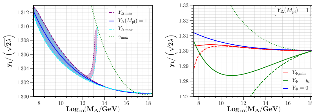
Figure 10. Predictions on the top Yukawa-Higgs quartic coupling ratio as a function of the intermediate scale M_\Delta . The relative change with M_\Delta can be directly translated to a prediction for the top-Higgs mass ratio if compared with the ratio for M_\Delta = M_{\text{pl}} , which is given by y_t/\sqrt{2}\lambda \sim 1.3004 . Left: change in the predictions due to the triplet only. The solid blue line refers to the value Y_\Delta(M_{\text{pl}}) = 1 and the dotted lines are the predictions corresponding to the lower and upper bounds on Y_\Delta derived from vacuum stability in section 3.4. The blue shaded region is the range of predictions allowed by vacuum stability with vanishing cubic coupling \gamma . The purple shaded region shows the prediction when \gamma is given by eq. (2.19) and the masses of the light neutrinos are due to a seesaw type II. The dotted green line correspond to |\gamma| = \gamma_{\text{max}} . Right: change in the predictions when right-handed neutrinos are taken into account. We fixed Y_\Delta(M_{\text{pl}}) = 1 . The red lines are the predictions corresponding to the lowest bound on Y_{\Phi,\text{min}} derived from vacuum stability respectively in section 3.5. For the solid red line we use \gamma(M_{\text{pl}}) = 0 and for the dashed red line we set \gamma(M_\Delta) = 0 . The green lines are the predictions corresponding to Y_\Phi(M_\Delta) = y_t(M_\Delta) . The solid green line obtains for \gamma(M_{\text{pl}}) = 0 , the dashed blue line uses \gamma(M_\Delta) = 0 and the dotted green line corresponds to the maximum bound \gamma_{\text{max}} in eq. (2.18). The latter would be exactly the same for the lowest bound Y_{\Phi,\text{min}} since it corresponds to the choice \lambda(M_\Delta) = 0 independent of Y_\Phi . The blue solid line corresponds to the case without right-handed neutrinos, as in the left figure.
