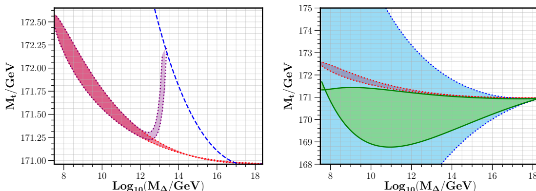
Figure 1. Predicted range in the top quark mass from asymptotically safe quantum gravity assuming a Higgs mass of M_H = 125.15 GeV. The predicted value of the top quark mass in the SM, M_t \sim 171 GeV, corresponds to the limiting case M_\Delta = M_{\text{pl}} . Left: in red we see the predicted bounds derived considering the SU(2) triplet alone and vanishing cubic coupling. In purple we present the bounds with the requirement that the mass of the light neutrinos mainly comes from the type II seesaw. The latter case implies bounds M_t \gtrsim 171.3 GeV and M_\Delta \lesssim 5 \times 10^{13} GeV. In blue we show the maximum value for the top mass using the maximum value of the cubic coupling allowed by vacuum stability. Right: the vacuum stability of the full Higgs double-triplet potential requires the presence of right-handed singlet neutrinos. In red we show again the bounds using the triplet alone and vanishing cubic coupling. In blue we illustrate how the bounds change if the neutrino-Higgs Yukawa coupling Y_\Phi is equal to the top-Higgs Yukawa coupling at the intermediate scale. The blue lower bound corresponds to a vanishing cubic coupling at the triplet scale. This bound depends on the value of Y_\Phi , with smaller Y_\Phi pushing the bound upwards. A shift of the bound in the same direction occurs if the right-handed neutrino masses are larger than the triplet mass. The blue upper bound corresponds to the maximum value that the cubic coupling can attain, for a vanishing quartic doublet coupling at the triplet scale M_\Delta . The solid green curves obtain for a vanishing cubic coupling at the Planck scale, for two values of the doublet-neutrino coupling Y_\Phi and right handed neutrino mass M_\nu = M_\Delta . For larger M_\nu the allowed interval in between the curves shrinks.
