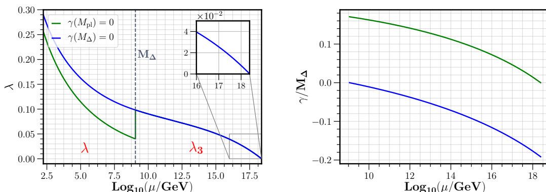
Figure 9. Left: running of the Higgs quartic coupling with the logarithm of the renormalisation scale in the type I+II seesaw using the 2-loop RGEs. We used the values given in eq. (3.1) for M_t = 170.97 \text{ GeV} as well as the extrapolation to M_{\text{pl}} described in the beginning of section 3. We required that \lambda_i(M_{\text{pl}}) = 0 with i = 1, 2, 3, 4, 5 and used M_{\Delta} = 10^9 \text{ GeV} , Y_{\Delta}(M_{\text{pl}}) = 1 and Y_{\Phi}(M_{\Delta}) = y_t(M_{\Delta}) which yields a stable doublet-triplet potential. The solid blue line corresponds to \gamma(M_{\Delta}) = 0 and the solid green line to \gamma(M_{\text{pl}}) = 0 . One finds \lambda, \lambda_3 > 0 for all \mu , leading to a stable vacuum. For \gamma(M_{\text{pl}}) = 0 (solid blue) there is a step between \lambda_3 and the effective Higgs quartic coupling \lambda at M_{\Delta} due to eq. (2.16). Right: running of the cubic coupling \gamma for the same example as in the left figure. The green and blue lines respectively corresponds to \gamma(M_{\text{pl}}) = 0 and \gamma(M_{\Delta}) = 0 .
