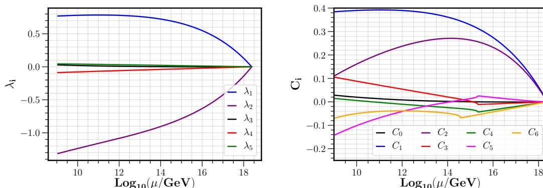
Figure 5. Running of the quartic couplings (left figure) and the conditions for the classical stability of the potential (right figure) for M_\Delta = 10^9 \text{GeV} and Y_\Delta(M_{\text{pl}}) = 1 , without right-handed neutrinos. Left: all quartic couplings vanish at the Planck scale. The running of \lambda_1 and \lambda_2 has opposite trends, and similar for \lambda_4 and \lambda_5 . This is due to the different sign of the contribution of the gauge and neutrino Yukawa couplings in eq. (3.8)–(3.11). Right: we display the values of the constraints C_i discussed in section 3.3, with a stable potential for positive C_i . The interaction of the triplet with left-handed leptons, Y_\Delta , stabilises the potential of the triplet alone, that is C_1, C_2 > 0 , even though \lambda_2 < 0 . The other conditions are in general not met. In particular, we have that C_5, C_6 < 0 evaluated at M_\Delta . Also we find that \lambda_3 < 0 for \mu \gtrsim 10^{15} GeV (see figure 3). This is the reason why the lines corresponding to C_i with i = 3, 4, 5, 6 change at \mu \gtrsim 10^{15} GeV. For these contributions we employ the real part of the square root of \lambda_3 in eqs. (3.19) and (3.20).
