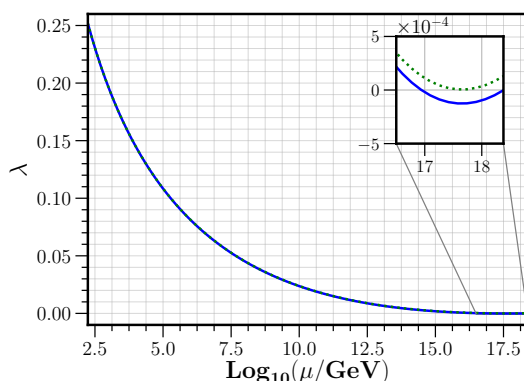
Figure 2. Running of the Higgs quartic coupling with the logarithm of the renormalisation scale \mu in the SM using the 2-loop RGEs. We used the values given in eq. (3.1) for M_t = 170.97 GeV (solid blue line) and M_t = 170.96 GeV (dotted green line). The difference between requiring \lambda(M_{\text{pl}}) = 0 or \lambda \geq 0 , respectively the solid blue and dotted green lines, only yields a tiny correction to \lambda or M_t .
