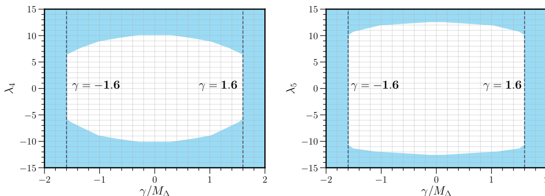
Figure 11. Unitarity bounds on the ratio \gamma/M_\Delta against \lambda_4 and \lambda_5 , including finite scattering energy.
