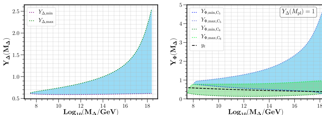
Figure 7. Constraints for Yukawa couplings of neutrinos. Left: allowed parameter space for the triplet Yukawa coupling Y_\Delta by vacuum stability of the triplet potential. The lower bound is roughly at Y_{\Delta,\min} \sim 0.6 . The effect of right-handed neutrinos has been neglected. Right: allowed parameter region for the doublet Yukawa coupling Y_\Phi by requiring vacuum stability of the doublet-triplet potential, with fixed Y_\Delta(M_{\text{pl}}) = 1 . The blue and green shaded regions respectively correspond to the case where C_5 and C_6 are satisfied. The two regions overlap for large enough M_\Delta . In black we show the value of the top yukawa coupling.
