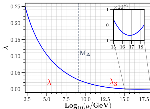
Figure 3. Running of the Higgs quartic coupling with the logarithm of the scale in the type II seesaw using the 2-loop RGEs. We used the values given in eq. (3.1) for M_t = 170.97 GeV as well as the extrapolation to M_{\text{pl}} described in the beginning of section 3. We required that \lambda_i(M_{\text{pl}}) = \gamma(M_{\text{pl}}) = 0 with i = 1, 2, 3, 4, 5 and used M_\Delta = 10^9 GeV and Y_\Delta(M_{\text{pl}}) = 1 , which yields a stable triplet potential. The negative value of \lambda between \mu \sim 10^{15} - 10^{18} GeV makes the stability issue a bit worse than in the SM. Right-handed neutrinos help stabilise the vacuum.
