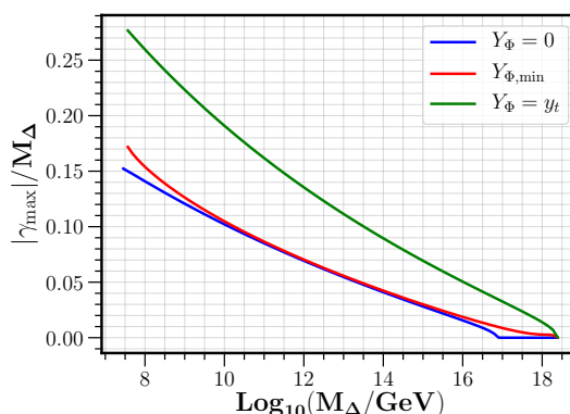
Figure 8. Maximum bound on the cubic coupling |\gamma| by requiring vacuum stability below M_\Delta , i.e. \lambda(M_\Delta) > 0 , as a function of the triplet mass. In blue, red and green we respectively show the cases of Y_\Phi(M_\Delta) = \{0, Y_{\Phi,\min}, y_t\} . The larger the Yukawa coupling Y_\Phi , the larger the maximum bound of |\gamma| . This is due to the fact that \lambda_3 grows faster with decreasing scale for larger Y_\Phi , see eq. (3.7).
