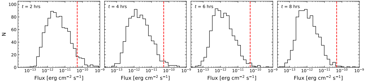
Fig. 7. Flux distribution of GRBs observed by Swift -XRT with T_{90} > 4 s (long bursts only) at two hours (left), four hours (middle left), six hours (middle right), and eight hours (right) after the initial outburst began. The red dashed line indicates a flux of 5 \times 10^{-11} erg cm ^{-2} s ^{-1} .
