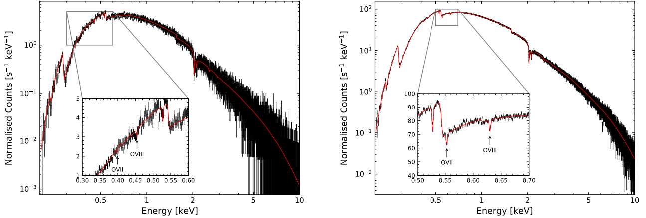
Fig. 1. 50 ks simulated X-IFU energy spectra of a GRB afterglow ( z_{\text{GRB}} = 2 ) imprinted by O VII ( \text{EW}_{\text{O VII}} = 0.35 eV) and O VIII ( \text{EW}_{\text{O VIII}} = 0.23 eV) WHIM absorbers. Both spectra are binned using the optimal binning scheme of Kaastra & Bleeker (2016). Left: GRB absorbed starting flux 5 \times 10^{-12} erg cm ^{-2} s ^{-1} and z_{\text{WHIM}} = 0.4388 . Right: GRB absorbed starting flux 1 \times 10^{-10} erg cm ^{-2} s ^{-1} and z_{\text{WHIM}} = 0.0382 . The insets show the energy range around the WHIM absorption features. Note: The absorption feature located at \approx 0.53 eV is the O resonance line of Galactic origin and is contained within the tbabs model component.
