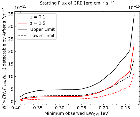
Fig. 8. Cumulative number of O VII–O VIII absorbers detectable by Athena per year above a minimum observed equivalent width for distributions of the WHIM at z = 0.1 (black) and z = 0.5 (red) as a function of the starting flux of the GRB afterglow and the predicted number of afterglows above that flux.
