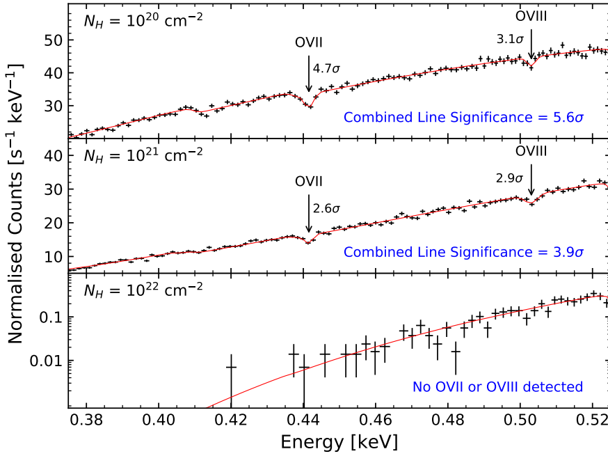
Fig. 5. Simulated X-IFU spectrum for varying Milky Way hydrogen column densities with O VII and O VIII absorption features at z_{\text{WHIM}}=0.3 . Input lines have equivalent widths of \text{EW}_{\text{O VII}}=0.28 eV and \text{EW}_{\text{O VIII}}=0.19 eV. Afterglow spectra have a starting flux of F_{\text{start}}=5 \times 10^{-11} erg cm ^{-2} s ^{-1} . Top : hydrogen column density of 10^{20} cm ^{-2} . Middle : hydrogen column density of 10^{21} cm ^{-2} . Bottom : hydrogen column density of 10^{22} cm ^{-2} .
