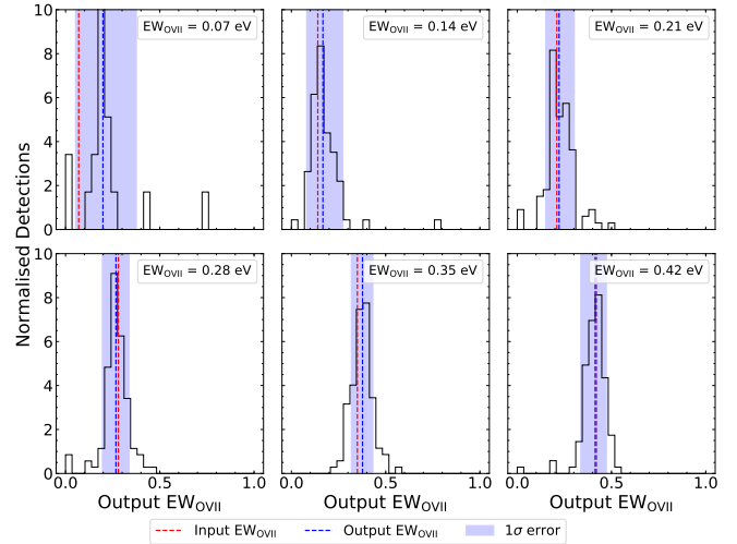
Fig. 4. Distributions of the fitted O VII equivalent widths in eV for each input O VII equivalent width from GRB afterglow spectra with F \geq 5 \times 10^{-11} \text{ erg cm}^{-2} \text{ s}^{-1} . The input equivalent width is represented by the red dashed line and the median equivalent width of the distribution is shown by the blue dashed line. The blue shaded area is the 1\sigma interval of the distribution.
