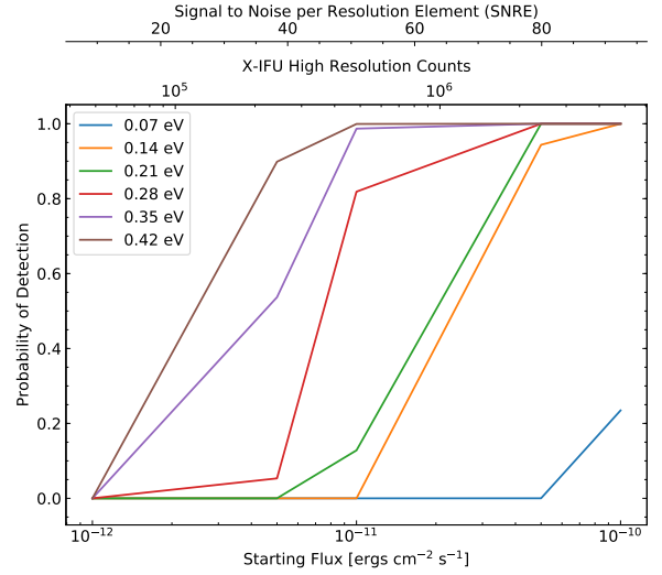
Fig. A.1. Detection probability of an unresolved absorption feature of a given equivalent width for GRB afterglow starting fluxes of 1, 5, 10, 50, and 100 \times 10^{-12} \text{ erg cm}^{-2} \text{ s}^{-1} .
