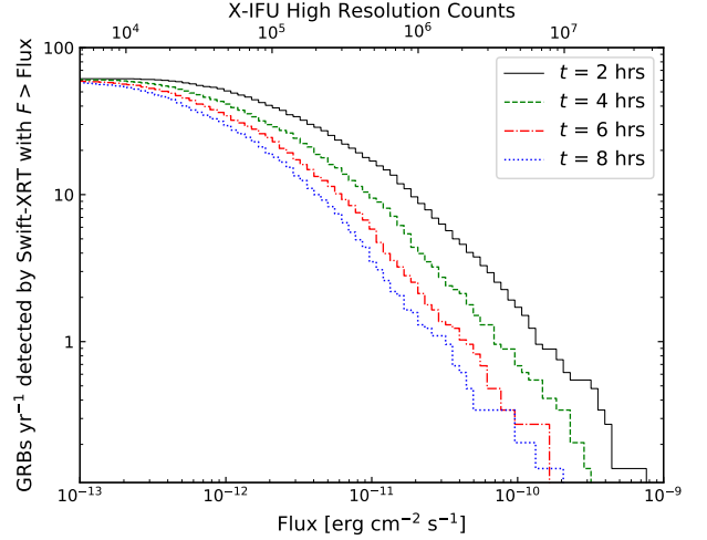
Fig. 9. Cumulative number of GRBs afterglows detected per year by Swift -XRT with T_{90} > 4 s (long bursts only) as a function of flux and X-IFU counts for observations made at two, four, six, and eight hours after the initial outburst began.
