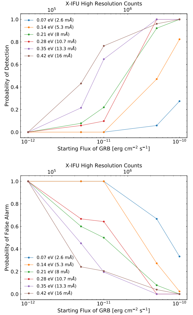
Fig. 2. Top: detection probability by O VII and O VIII absorption features for each EW simulated in the 35 mm defocused configuration of the Athena mirror. Bottom: false-alarm probability of WHIM detection by O VII and O VIII absorption features for each EW simulated EW in the 35 mm defocused configuration of the Athena mirror. EWs listed are those of O VII.
