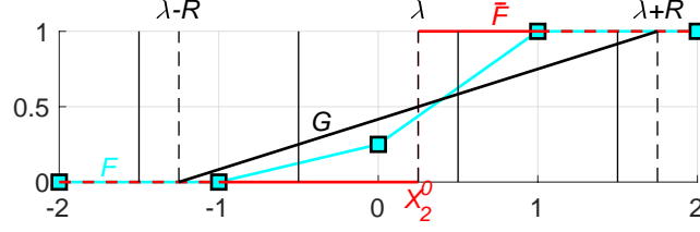
Figure 3: 1D VIC with perfect image.
