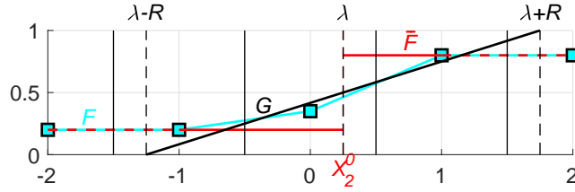
Figure 4: 1D VIC with reduced contrast but no brightness bias.
