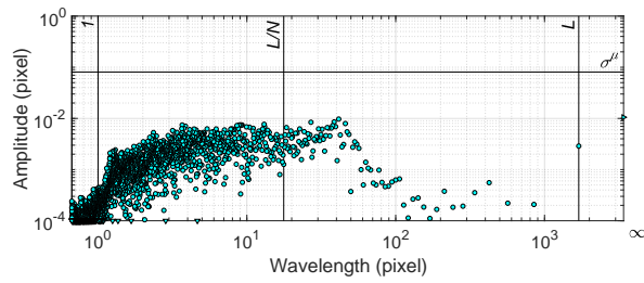
Figure 21: \text{FFT}(R\mu) for the steel ring image.
