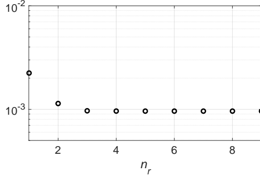
Figure 9: RMS deviation (pixel) as a function of the refinement parameter n_r , in average over \theta_0, X_{02}, \Delta L .
