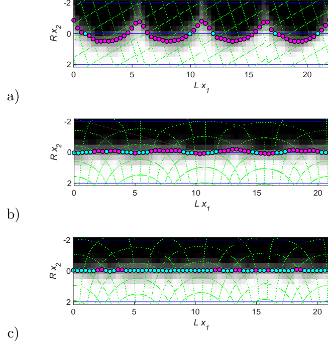
Figure 15: Images f of the small disc and its VIC measure with: a) square, b) 4-points B-spline of degree 2, c) circle. Circular marks: local identification R\mu , cyan if < \sigma^\mu , magenta if > \sigma^\mu . Green dotted lines: deformed pixel grid.
