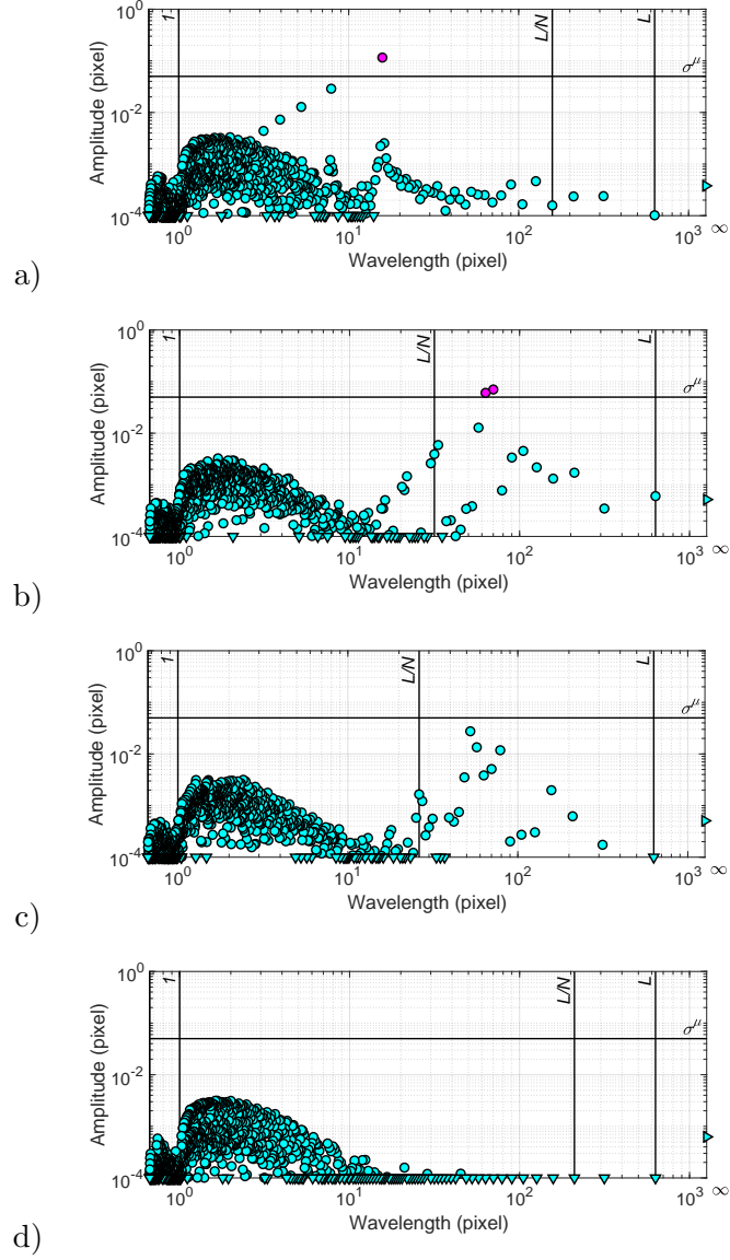
Figure 17: \text{FFT}(R\mu) for the large disc measured by: a) 40-sides regular polygon, b) 10-points B-Spline of order 2, c) 12-points B-Spline of order 2, d) circle.
