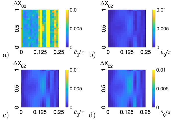
Figure 8: RMS deviation (pixel) for the line segment test with interpolation method a) nearest, b) linear, c) cubic, d) B-Spline.
