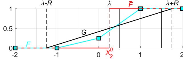
Figure 3: 1D VIC with perfect image.
