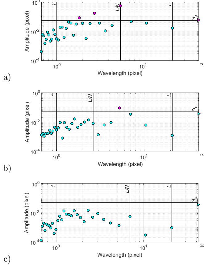
Figure 16: \text{FFT}(R\mu) for the small disc measured by: a) square, b) 4-points B-Spline of order 2, c) circle.
