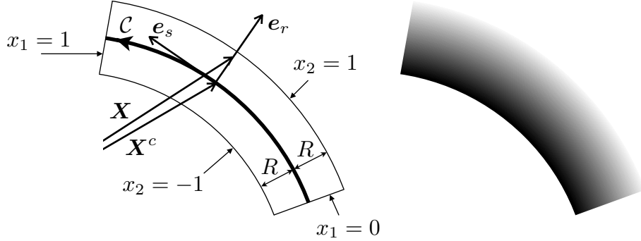
Figure 2: Virtual image geometry (left) and grey levels (right)
