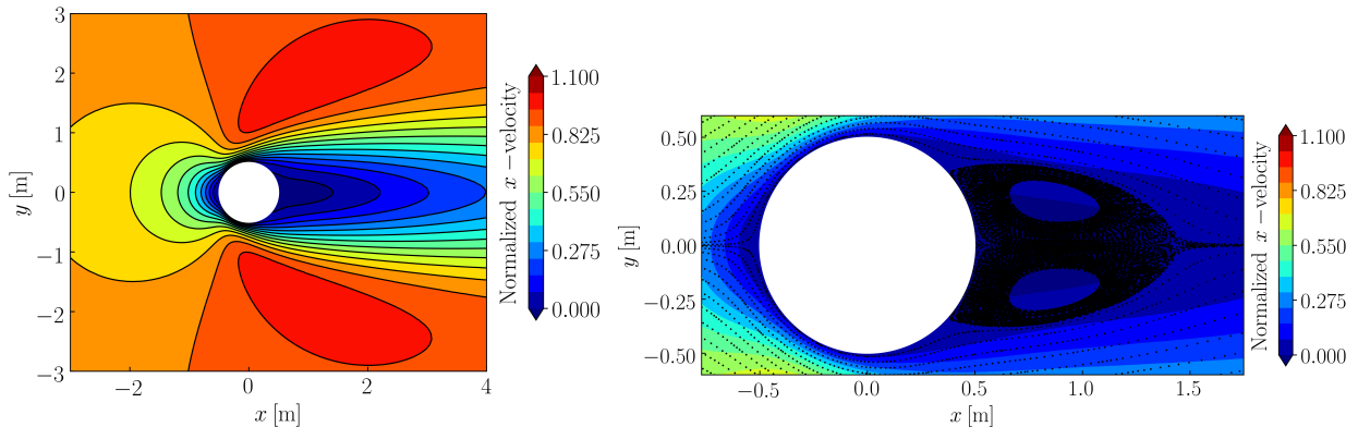
(a) Normalized x -velocity contours
