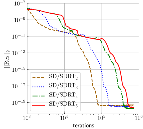
Figure 14: Convergence of the residual for the viscous flow around circular cylinder
