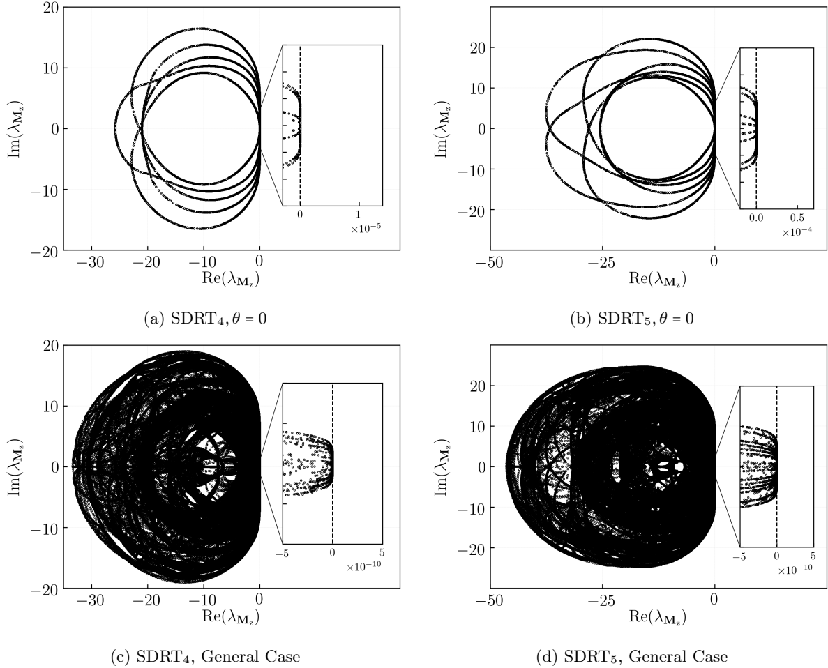
Figure 5: Fourier footprint of the SDRT 4 (left) and SDRT 5 (right) spatial discretizations on triangles
