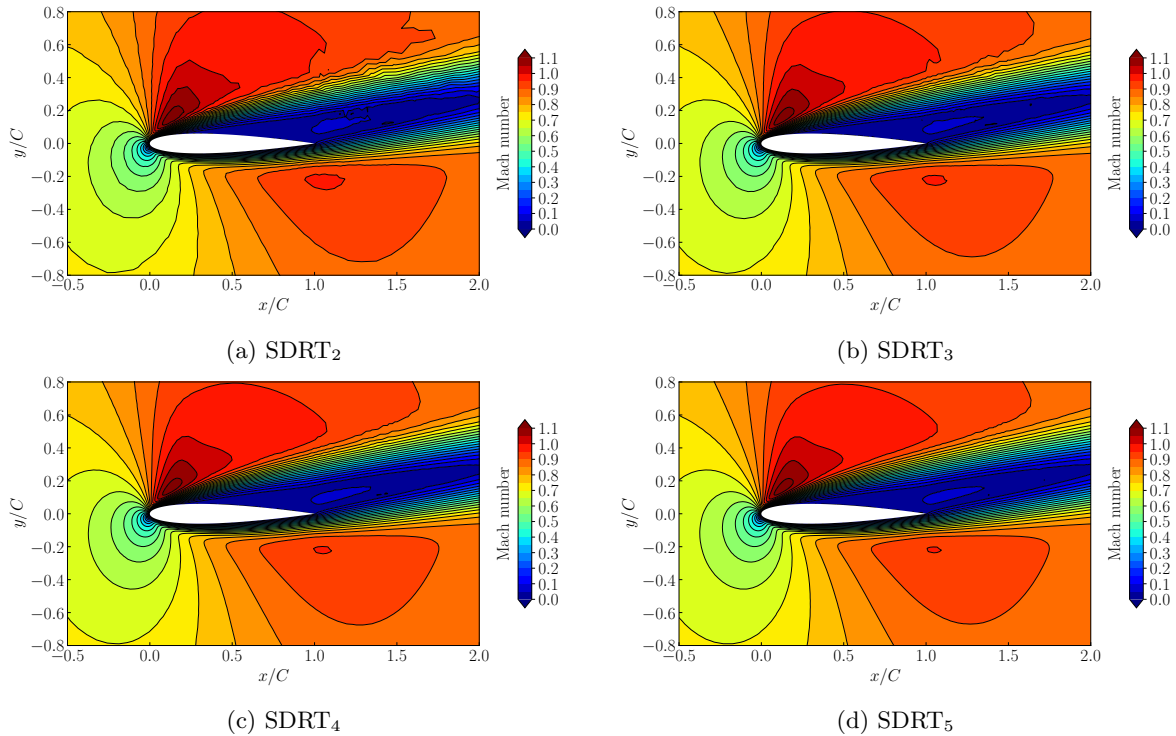
Figure 10: Case C: Mach number contours using SDRT p schemes, p \in \llbracket 2, 5 \rrbracket
