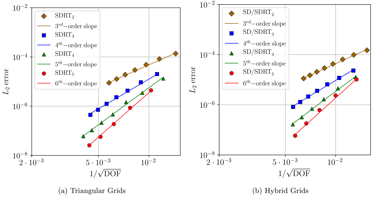
Figure 7: L_2 error and theoretical order of accuracy slopes for the COVO test case after 5 periods
