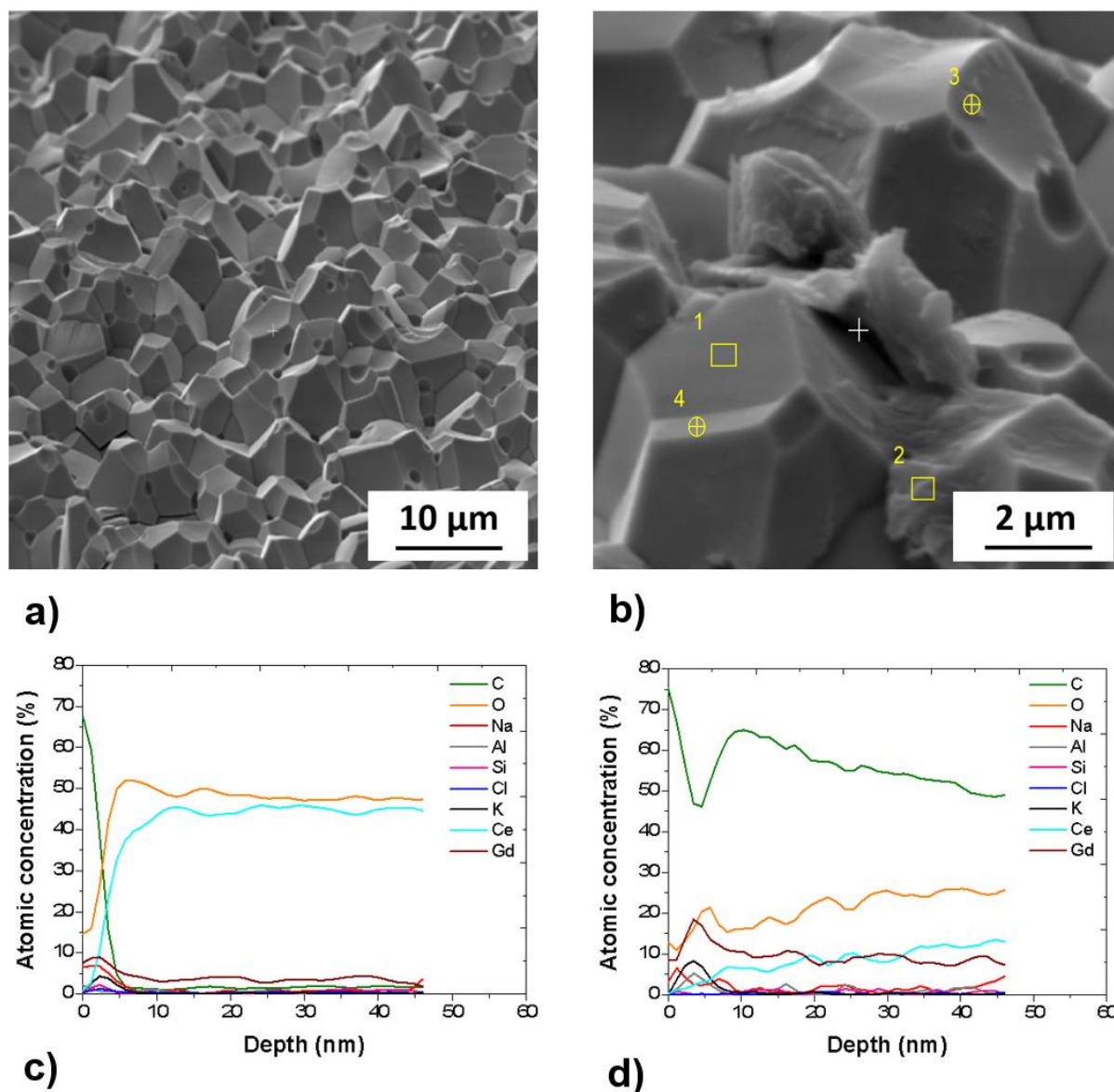
Figure 7: Chemical analysis performed by Auger Electron Spectroscopy (AES) in the grain and at the grain boundaries of GDC10 electrolyte obtained by tape casting: a) b) SEM images, c) analyses on the GDC grain for zone 1 (Fig. 8b) and d) at the grain boundaries for zone 2 (Fig. 8b).
