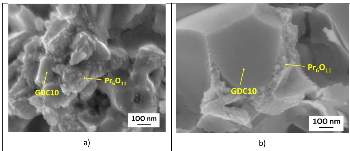
Figure 8 – Images of sections showing Pr 6 O 11 infiltration in a) die-pressed / screen-printed sample, b) tape-casted sample
