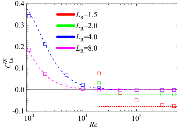
FIG. 22. Comparison of numerical predictions for C_{L_u}^W ( \square ) with the fit (15) of the asymptotic solution corresponding to conditions L_u \gg 1 , L_w \gg 1 (dashed lines), and the irrotational solution (17) (short-dashed lines), for 1.5 \leq L_R \leq 8 and 0.1 \leq Re \leq 500 .
