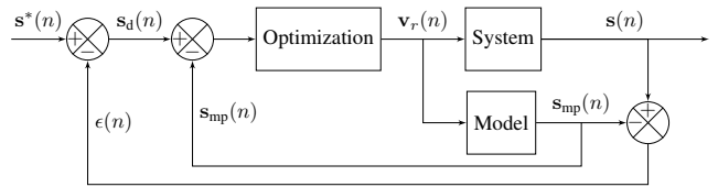
Fig. 5. Control structure [23]
